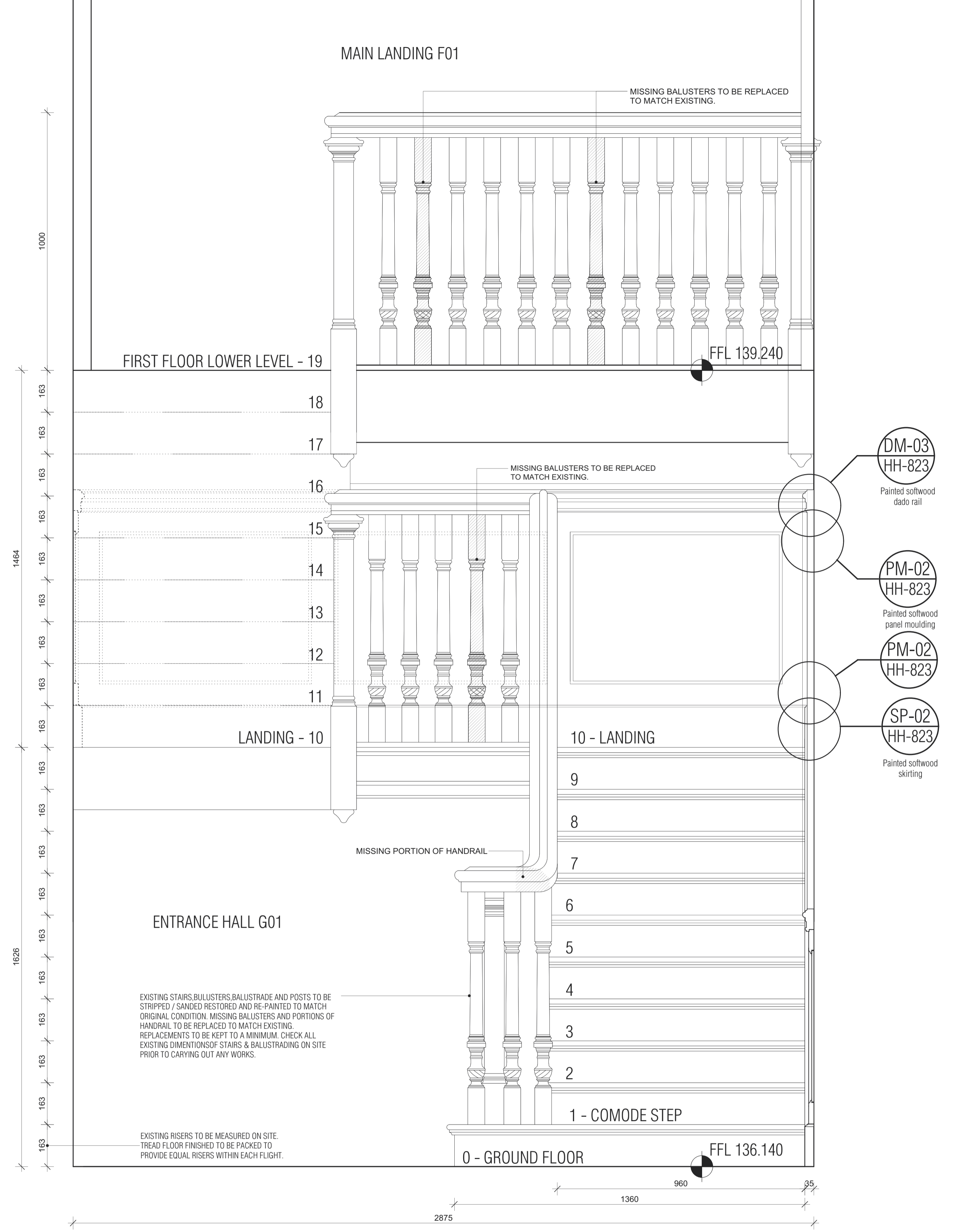
EXISTING GROUND TO FIRST FLOOR STAIRCASE & BALLUSTRADING RESTORATION ELEVATION 1/3 1:10
