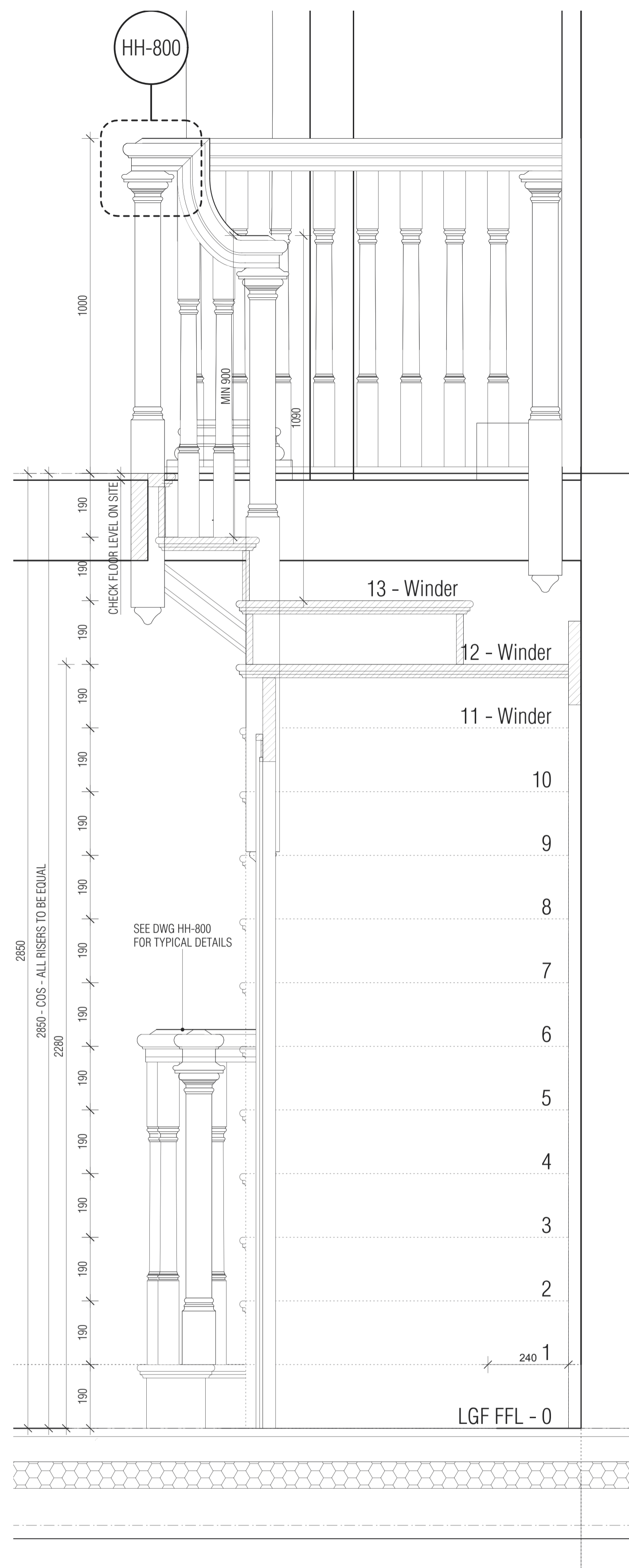
NEW LOWER GROUND TO GROUND FLOOR STAIRCASE ELEVATION 1/2 1:10
