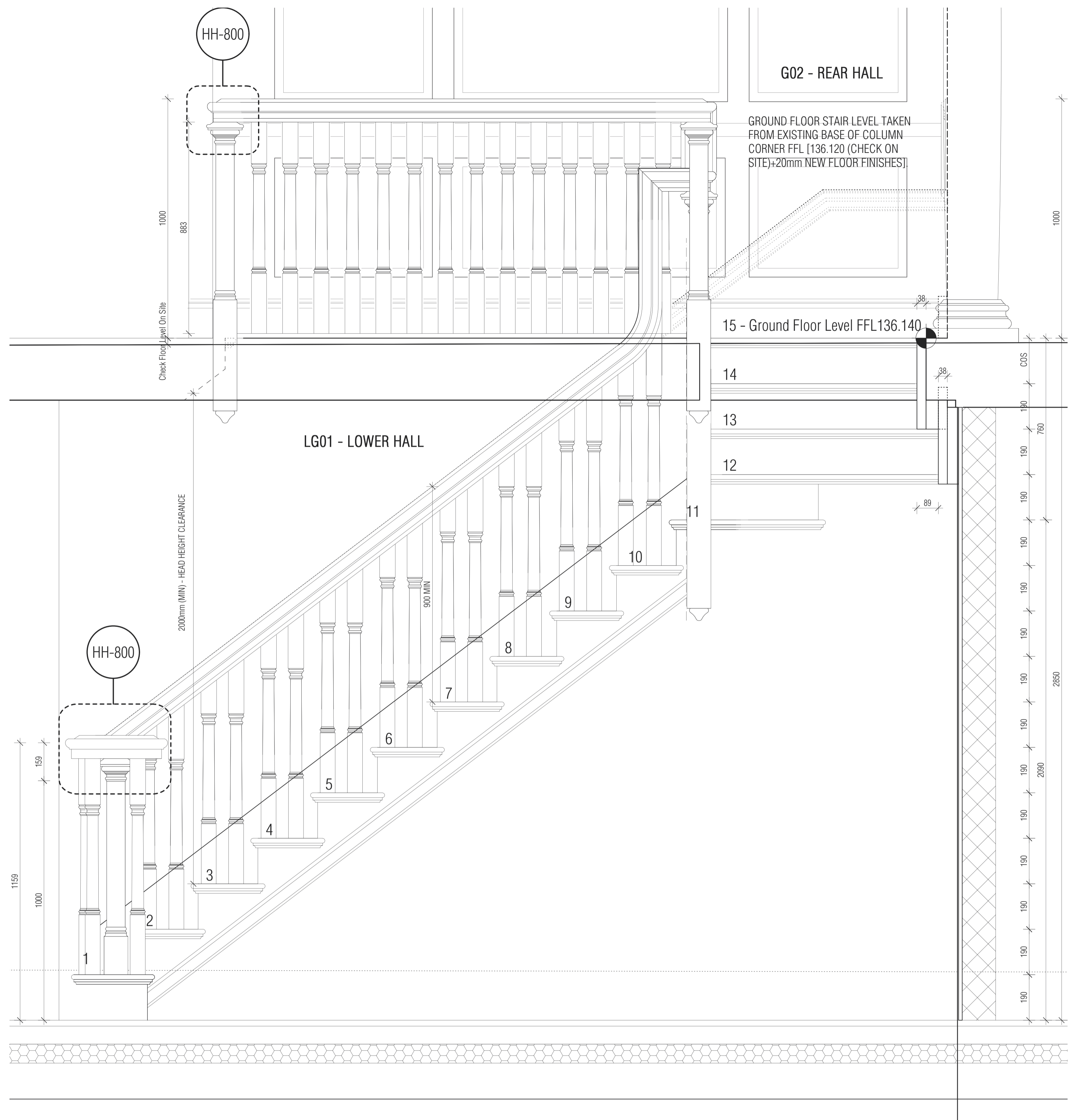
NEW LOWER GROUND TO GROUND FLOOR STAIRCASE ELEVATION 2/2 1:10
