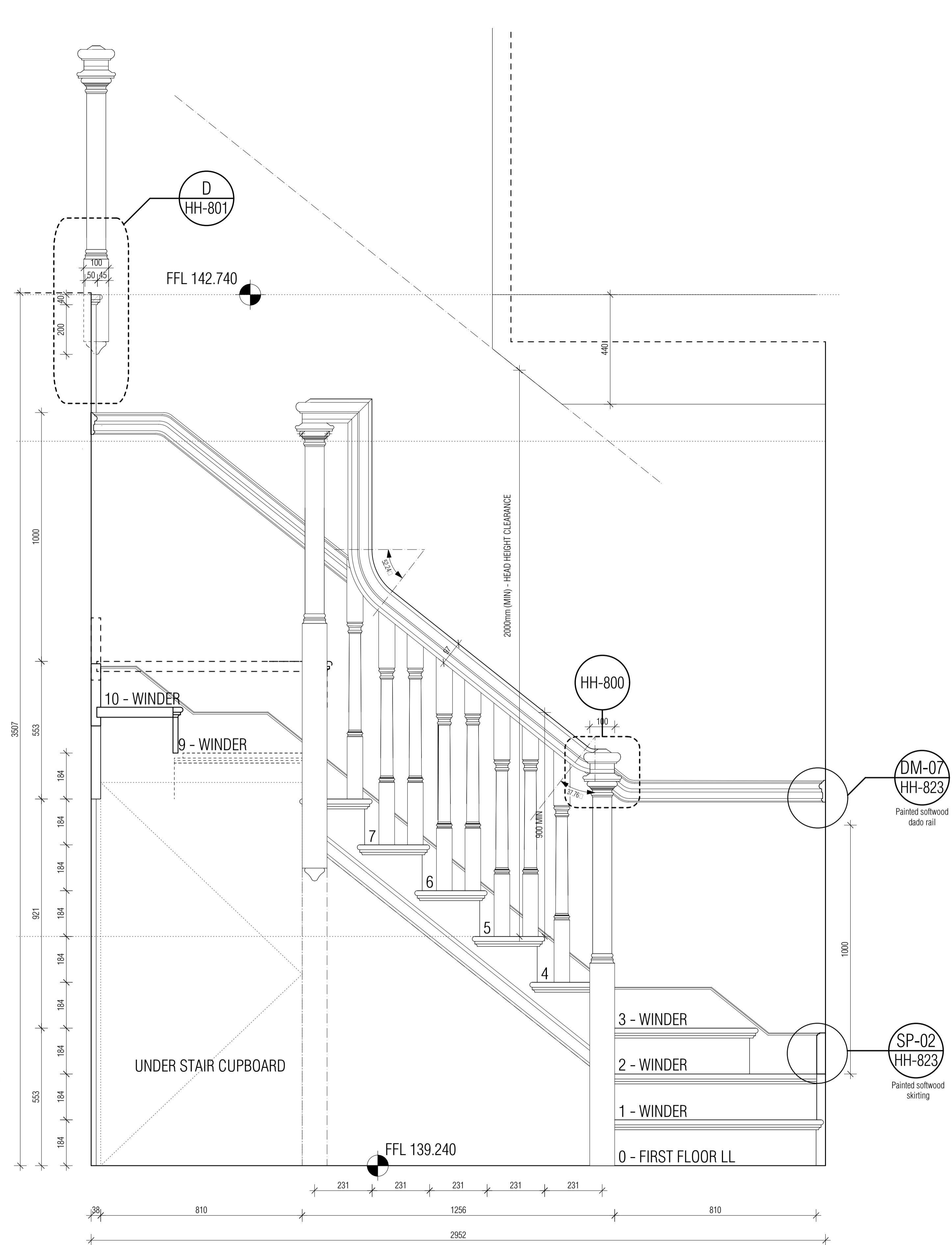
FIRST TO SECOND FLOOR STAIRCASE & SET OUT ELEVATION 2/3 1:10
