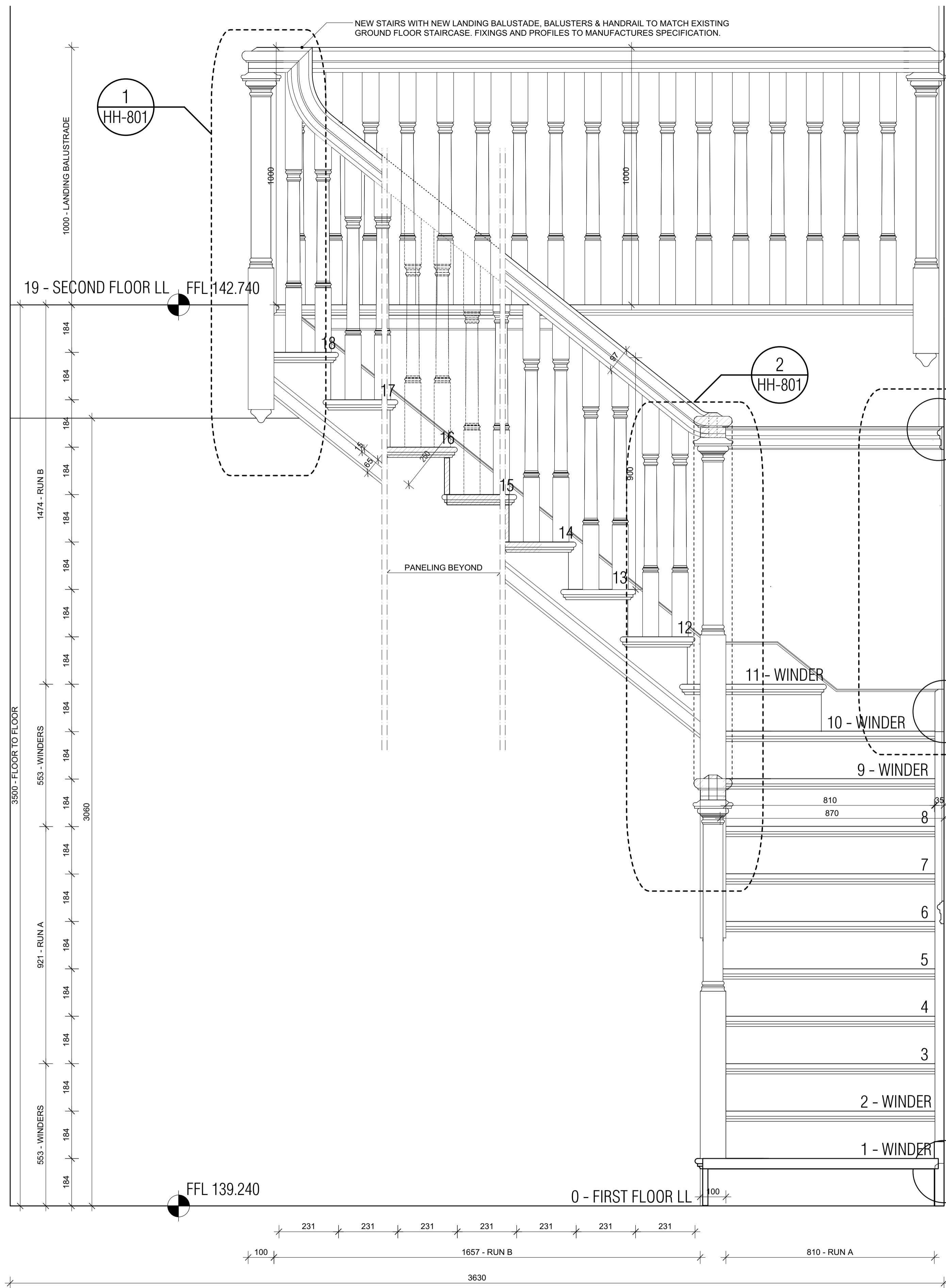
FIRST TO SECOND FLOOR STAIRCASE & SET OUT ELEVATION 1/3 1:10
