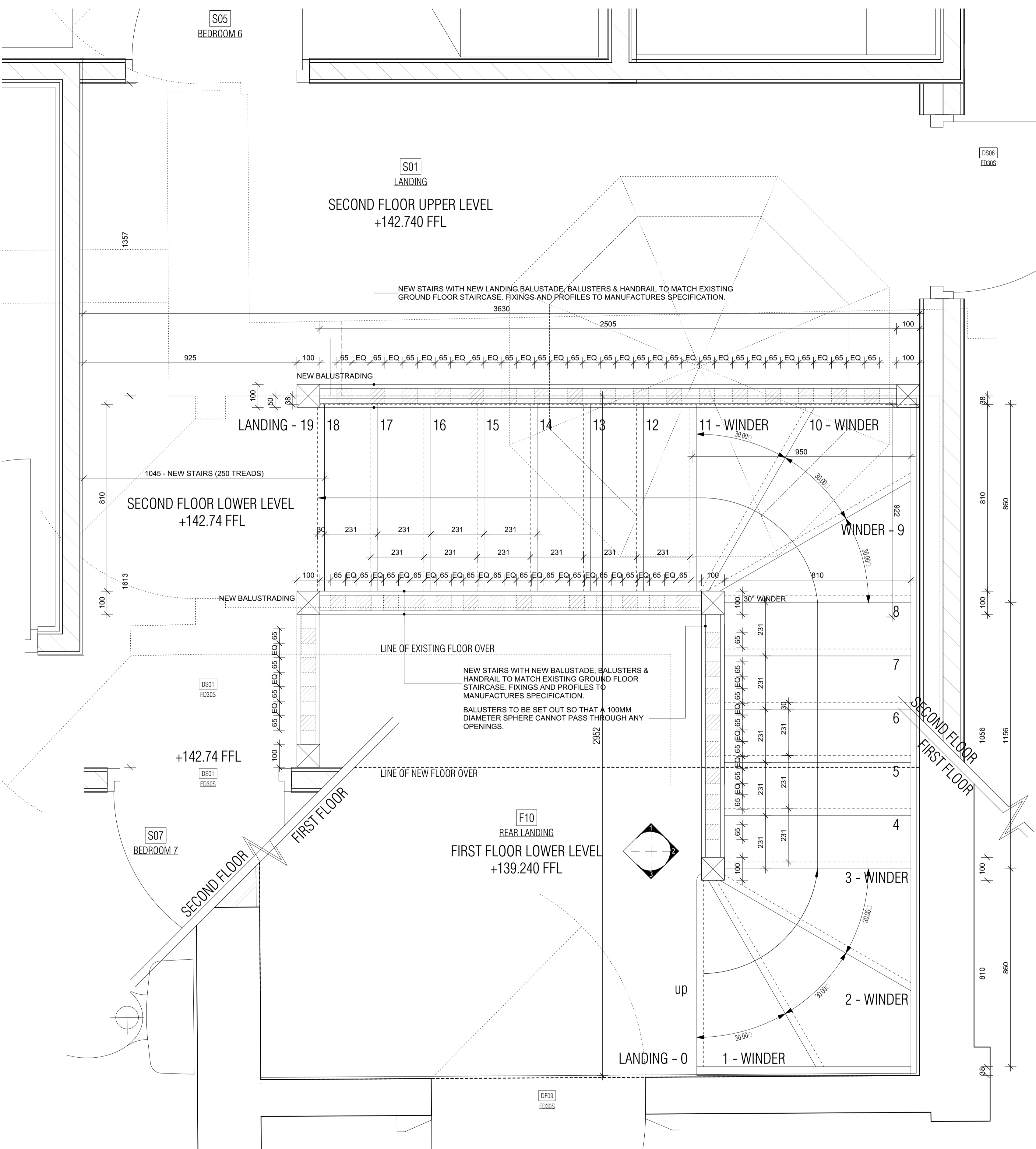
FIRST TO SECOND FLOOR STAIRCASE & BALLUSTRADING PLAN 1:10
