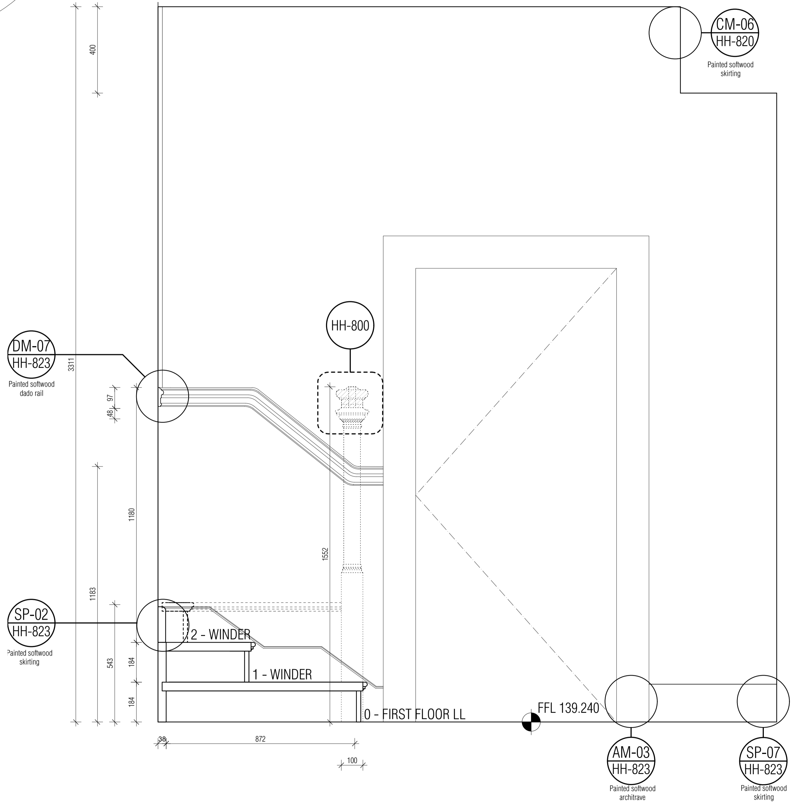
FIRST TO SECOND FLOOR STAIRCASE & SET OUT ELEVATION 3/3 1:10
