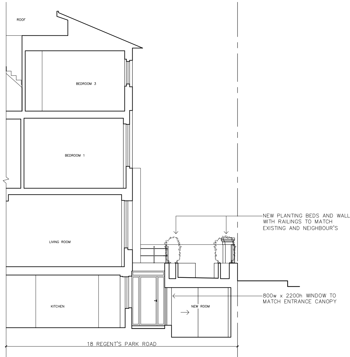
SECTION B - THROUGH PLANTING BEDS
