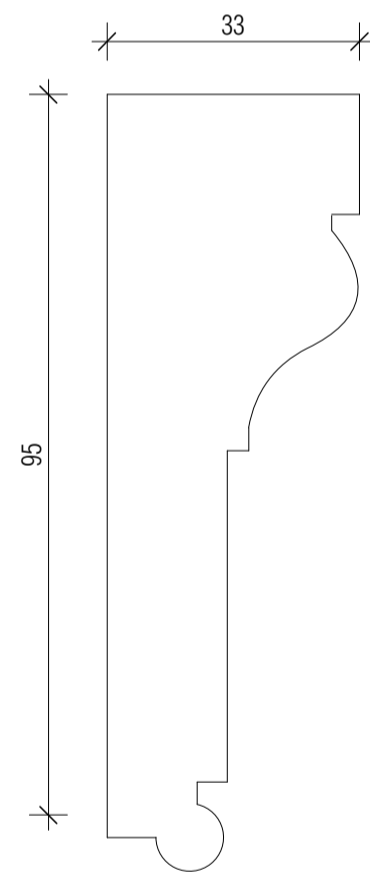
WAM02 Window Architrave Moulding 2 (based on pg.170; item 3; No.5-13 Queen Anne's Gate; 1770)
