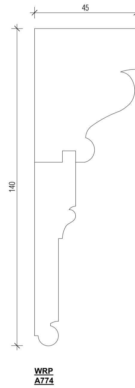
AM06 Door Architrave Moulding 6 (WRP-Timber mouldings - A774)
