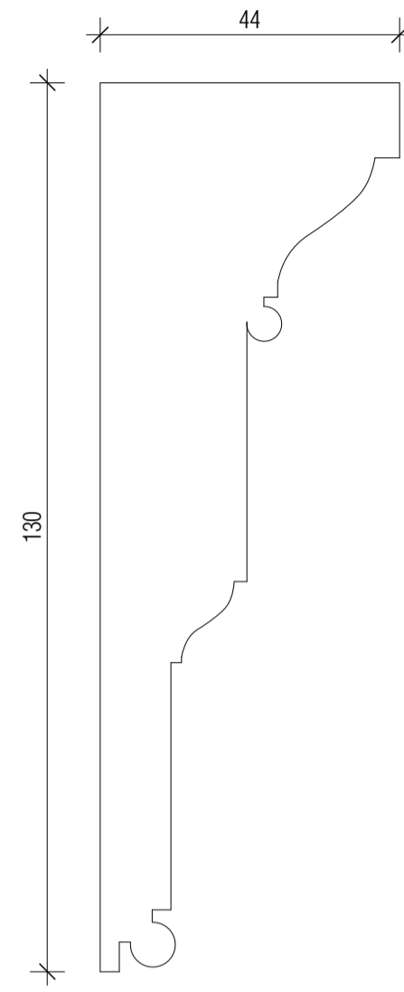
AM05 Door Architrave Moulding 5 (pg.170; item 2; No.5-13 Queen Anne's Gate; 1770)
