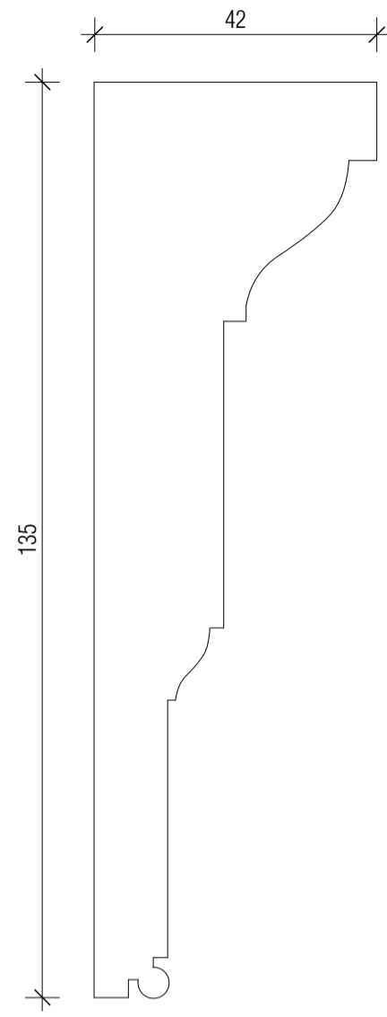
WAM01 Window Architrave Moulding 1 (pg.172; item 8; No.27 Fournier Street, Spitalfields; 1726)
