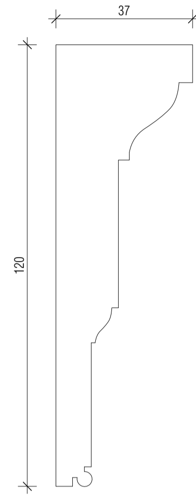
AM03 Door Architrave Moulding 3 (pg.170; item 1; Fournier Street, Spitalfields; 1726)
