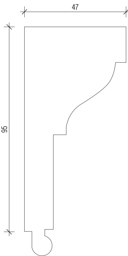
WAM01 Window Architrave Moulding 1 (pg.172; item 8; No.27 Fournier Street, Spitalfields; 1726)
