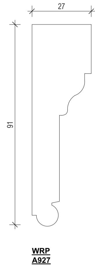
AM04 Door Architrave Moulding 4 (WRP-Timber mouldings - A927)
