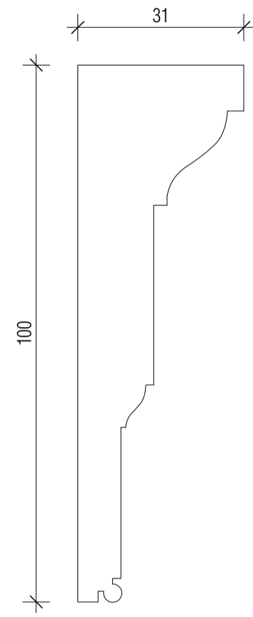
AM02 Door Architrave Moulding 2 (pg.170; item 1; Fournier Street, Spitalfields; 1726)
