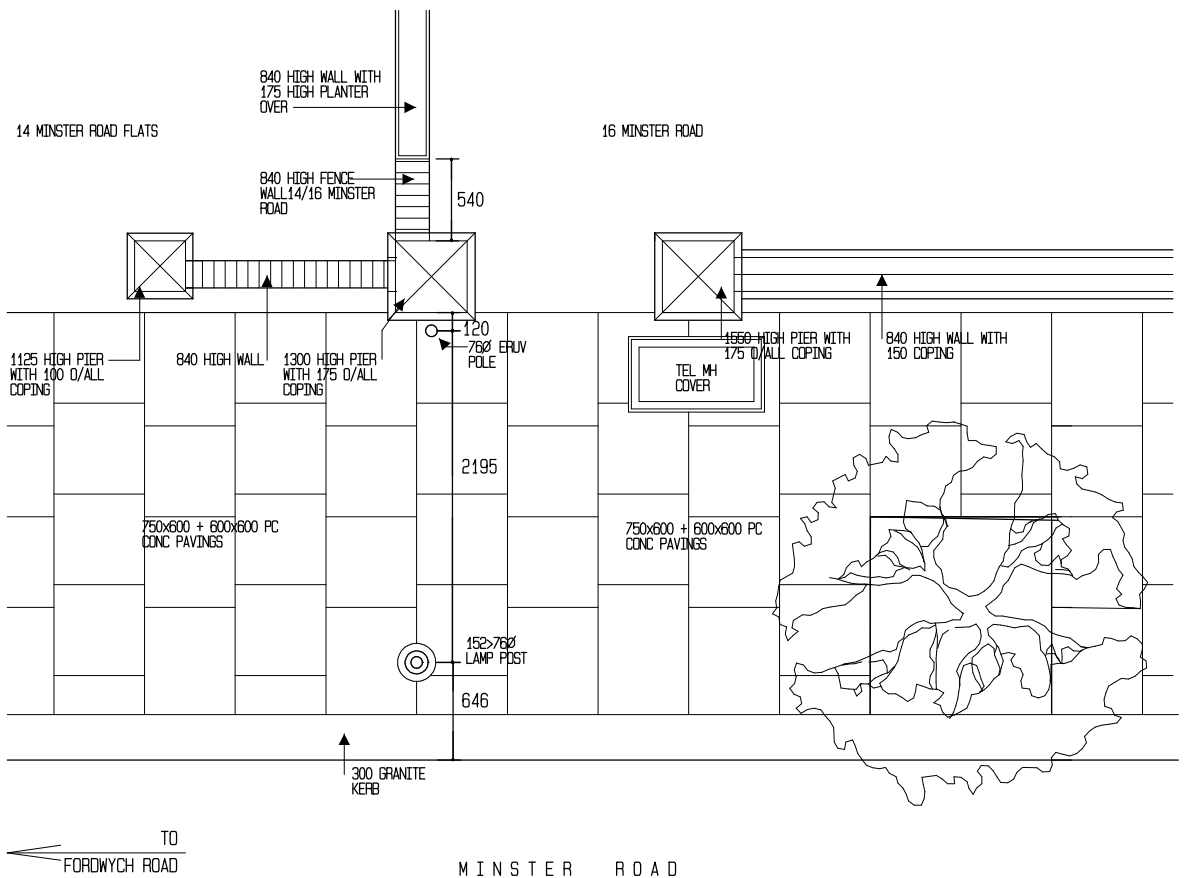
LOCAL PLAN -- MINSTER ROAD NW SIDE
