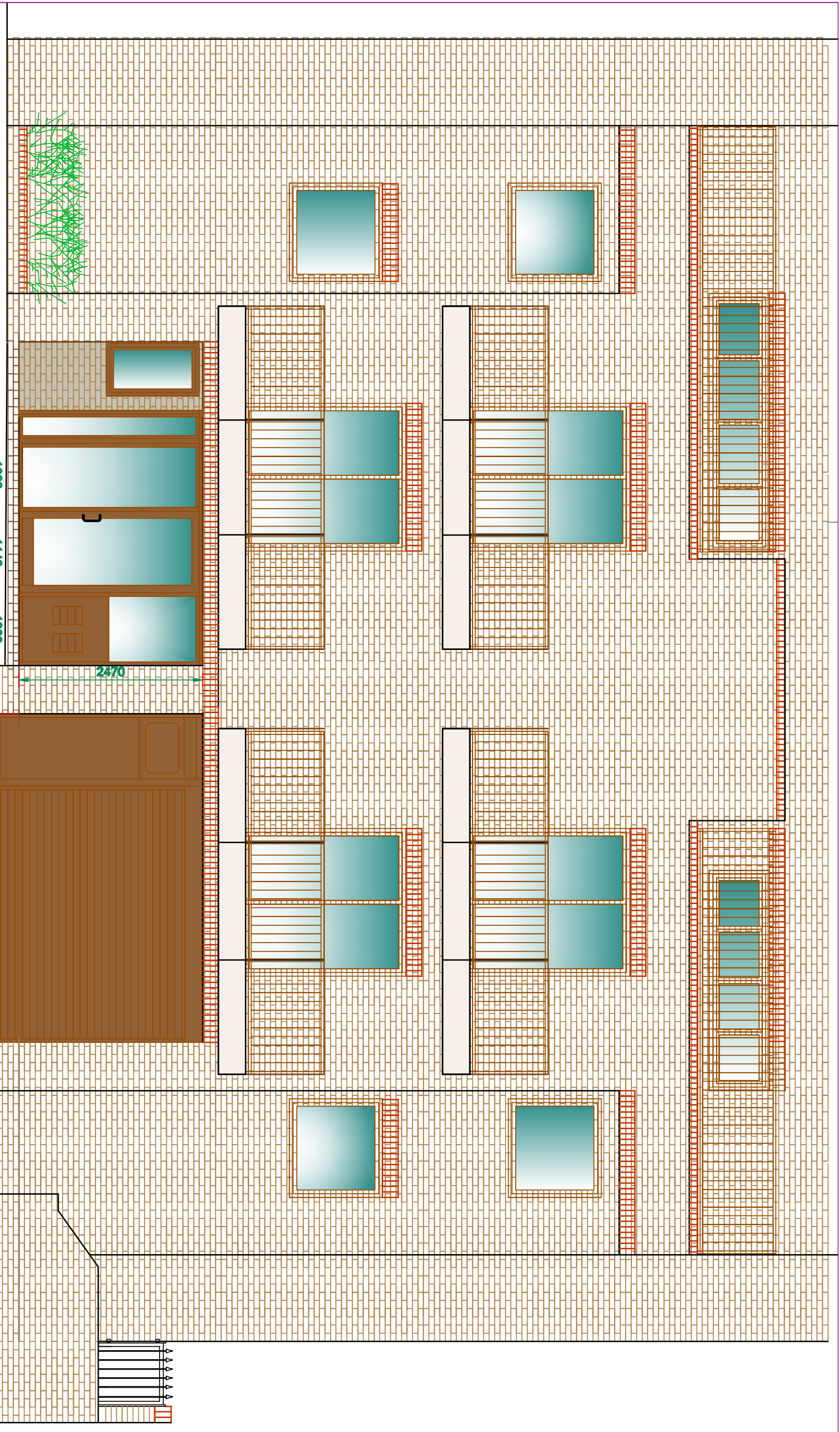
Drawing Title Proposed Front Elevation 1-50
