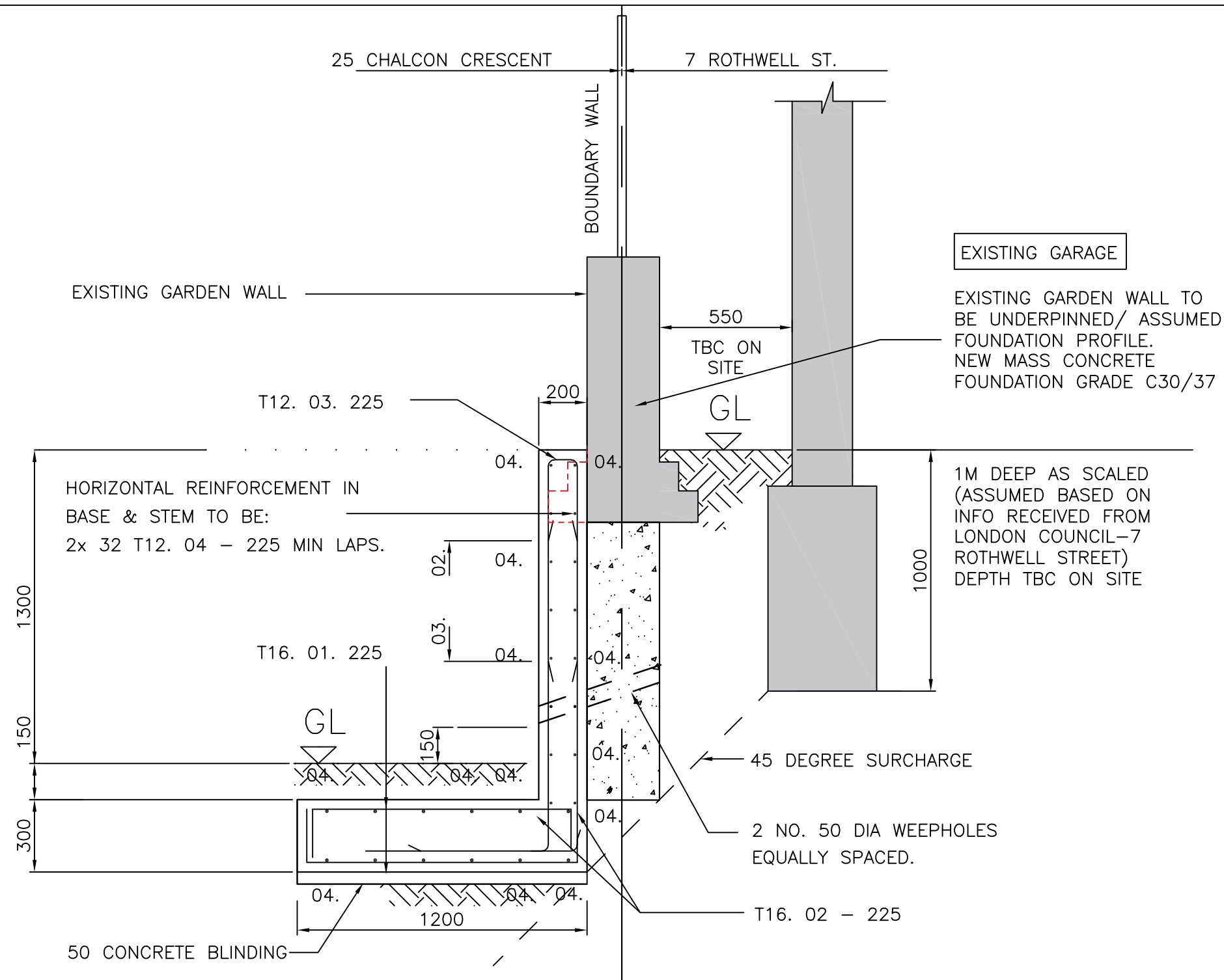
TYPICAL SECTION
