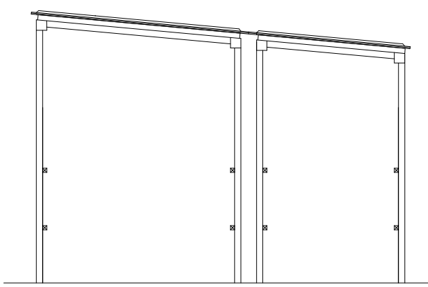
SECTION B-B
