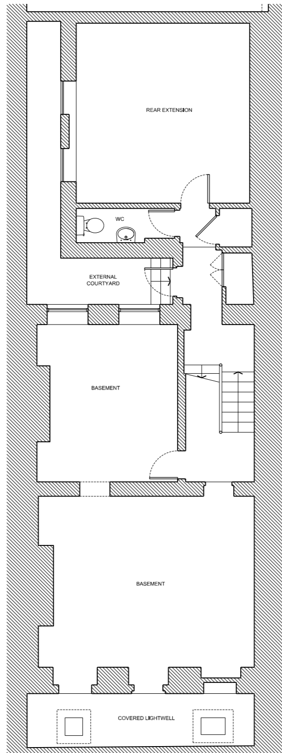
01 EXISTING GA PLAN 00 100 BASEMENT LEVEL PLAN 1:100
