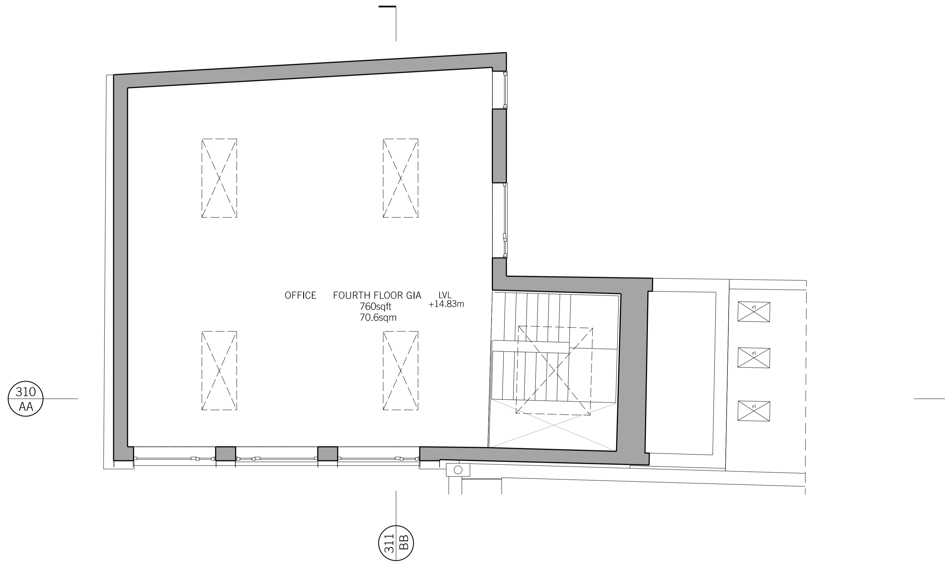
01: PROPOSED FOURTH FLOOR PLAN SCALE 1:50
