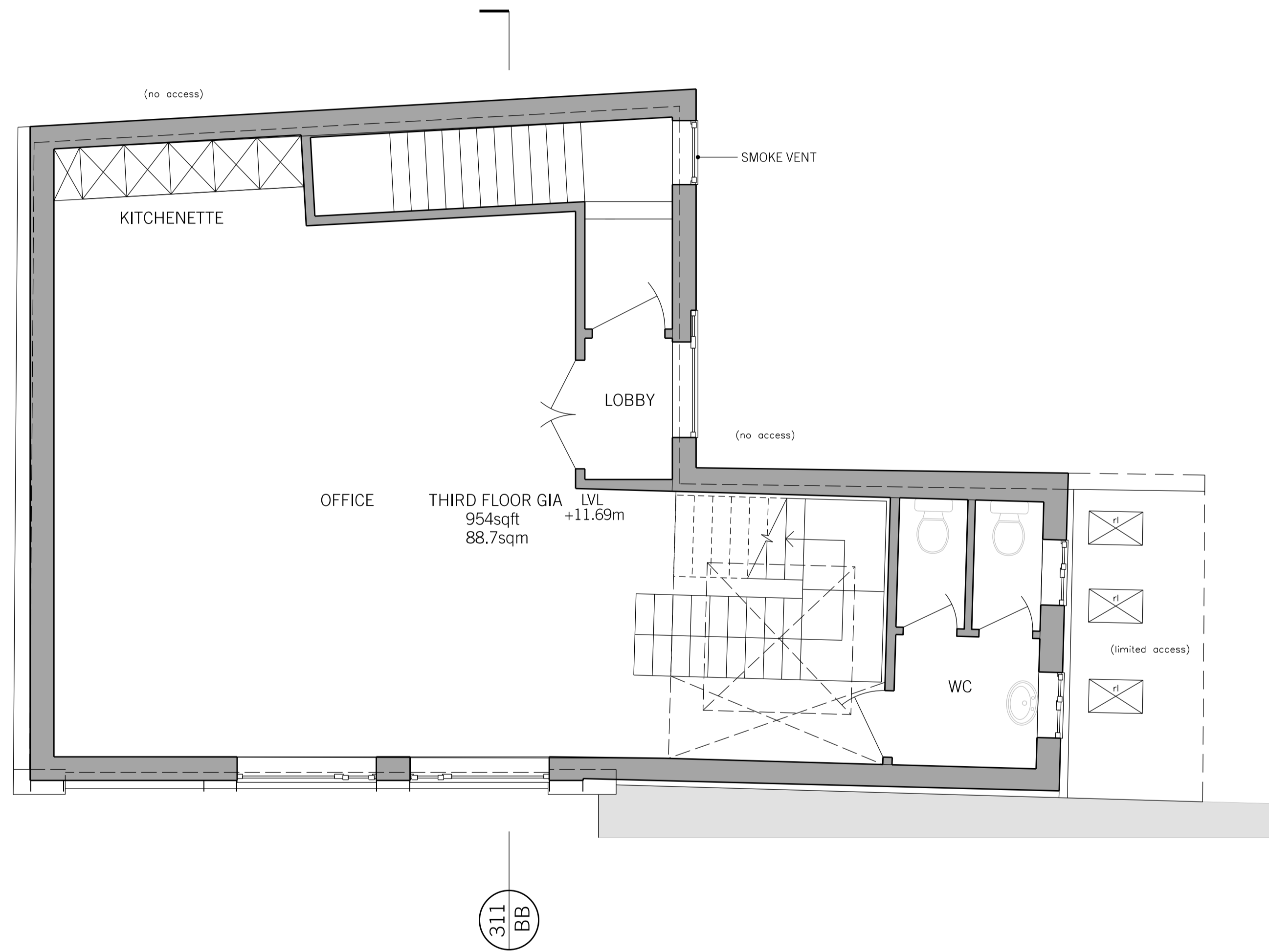
01: PROPOSED THIRD FLOOR PLAN SCALE 1:50
