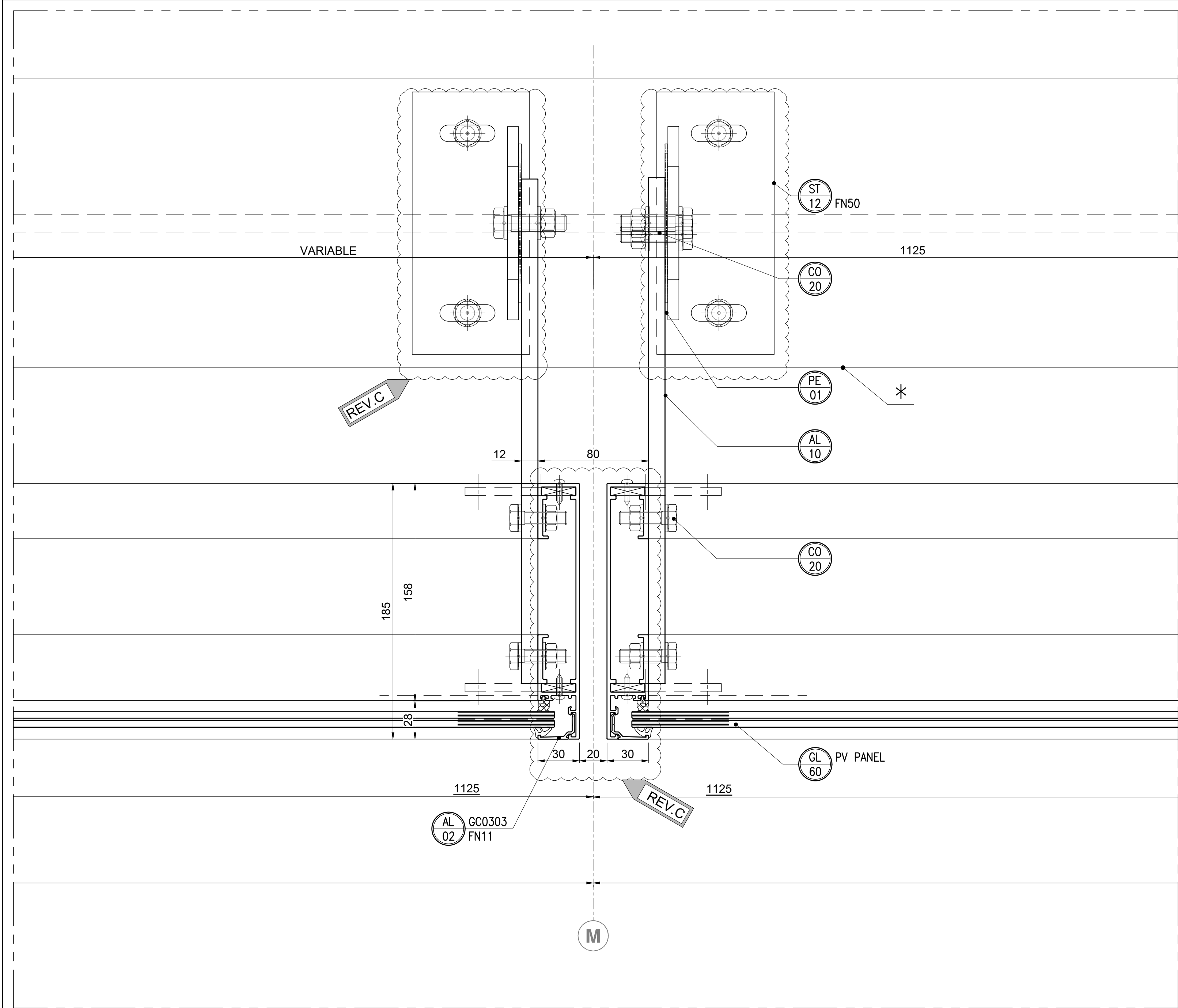
1 HORIZONTAL SECTION SCALE /1:2/
