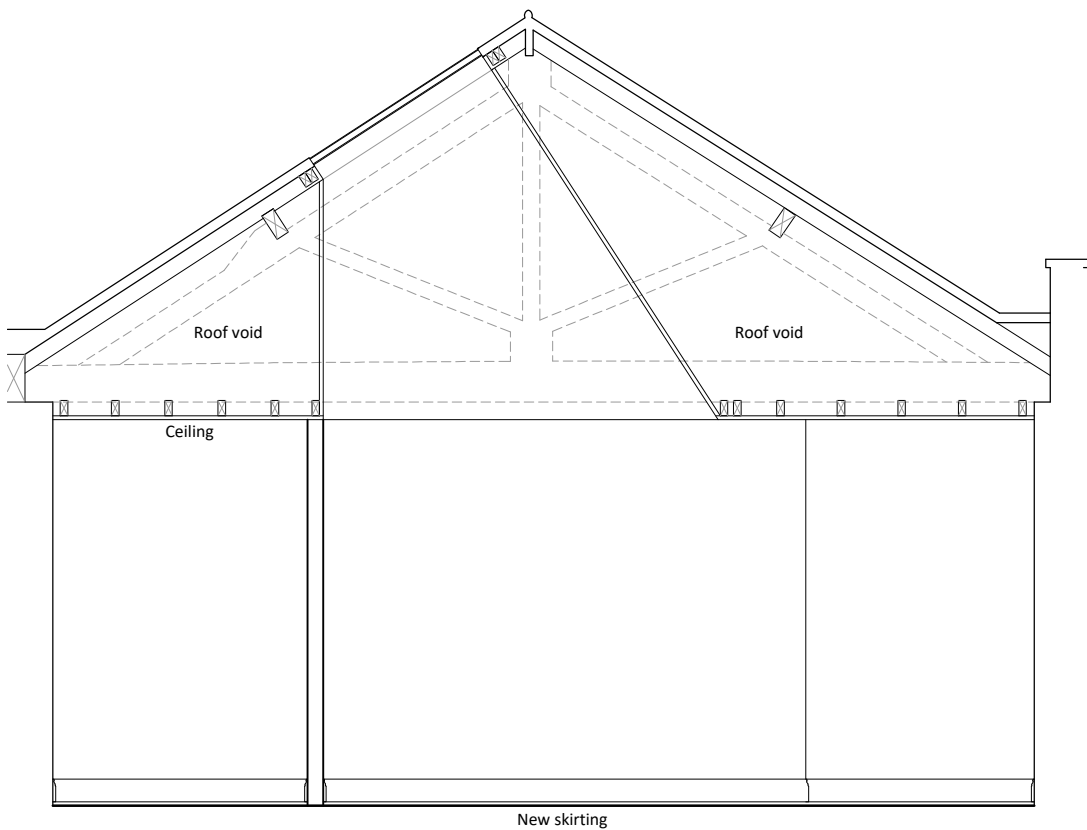
Elevation C
