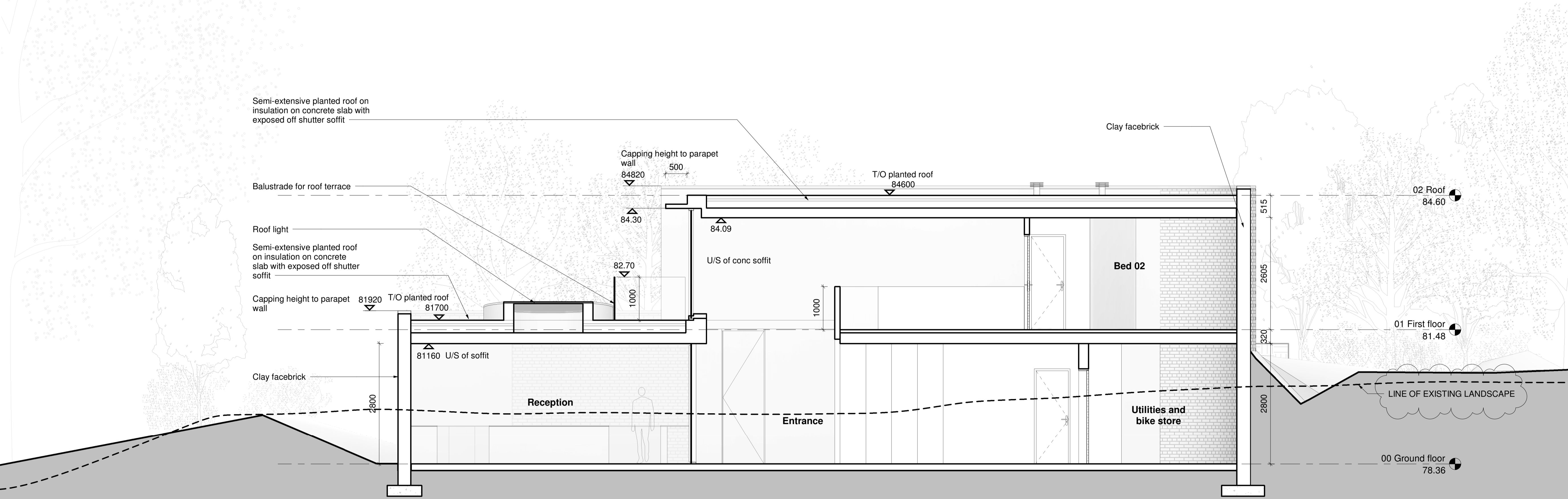
S2 Section S2 A2010 1:50 0 1m 5m 10m
