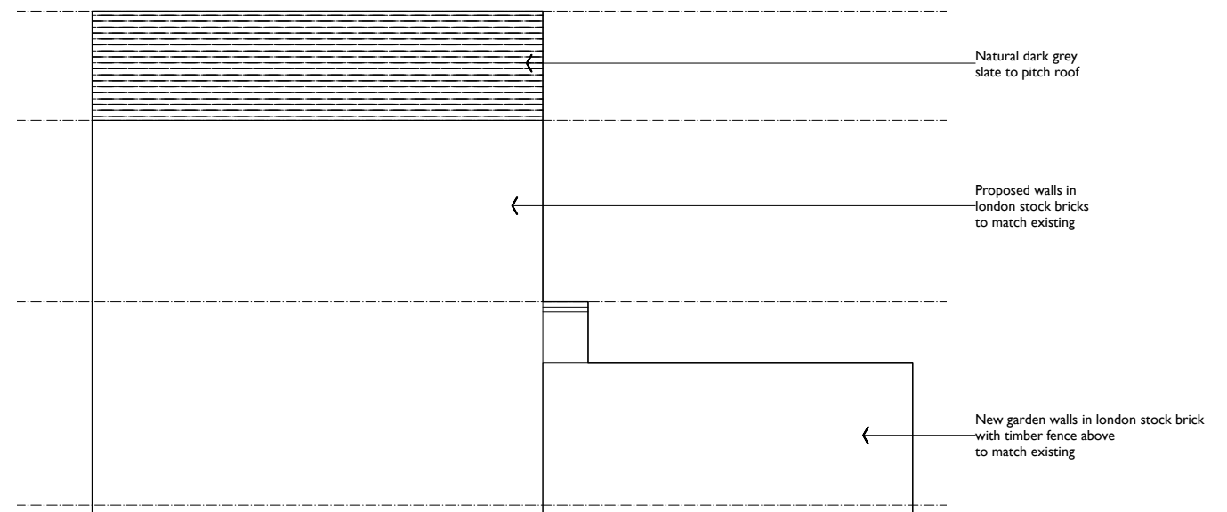
04 NORTH ELEVATION
