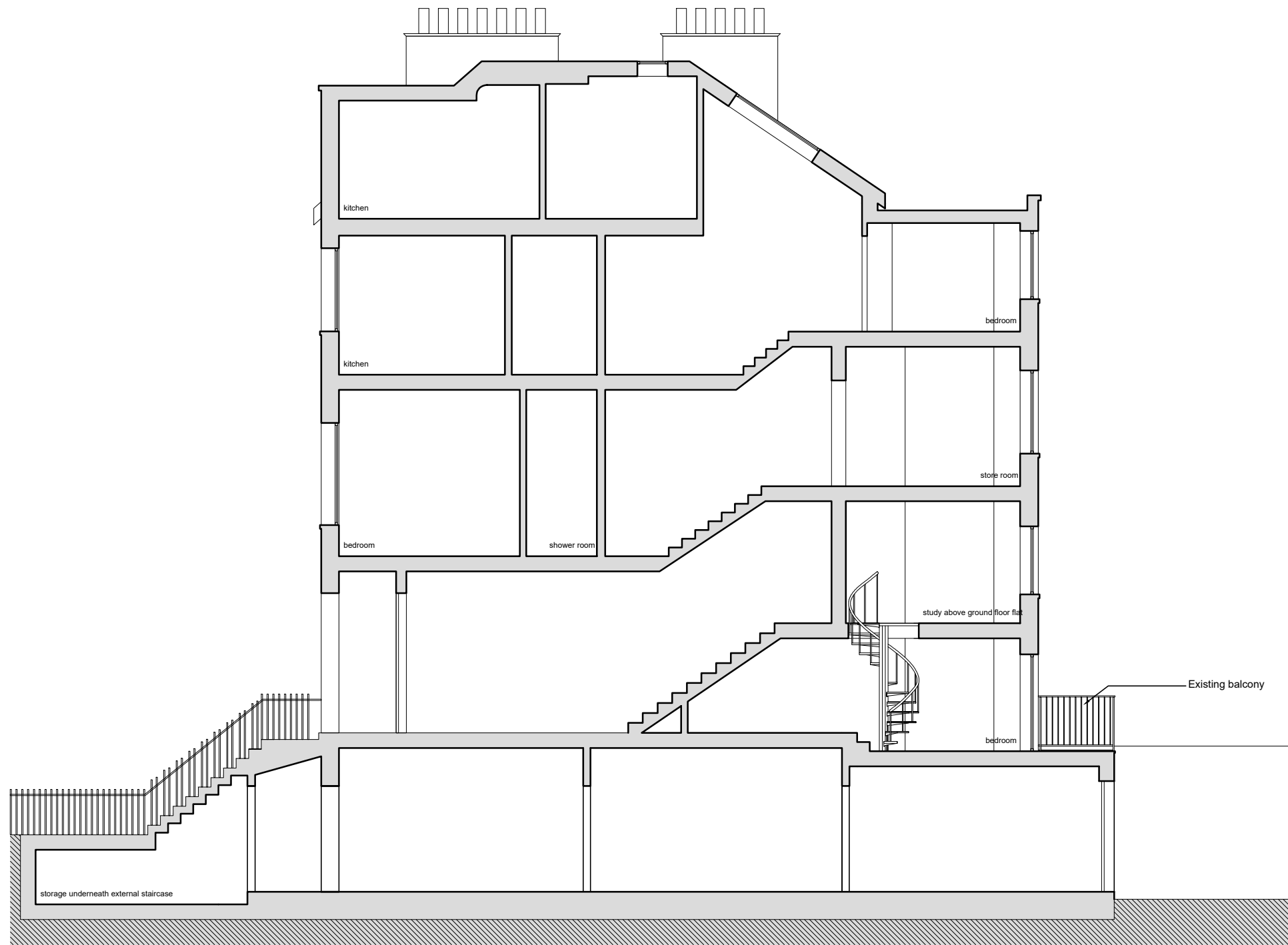
Section EE
