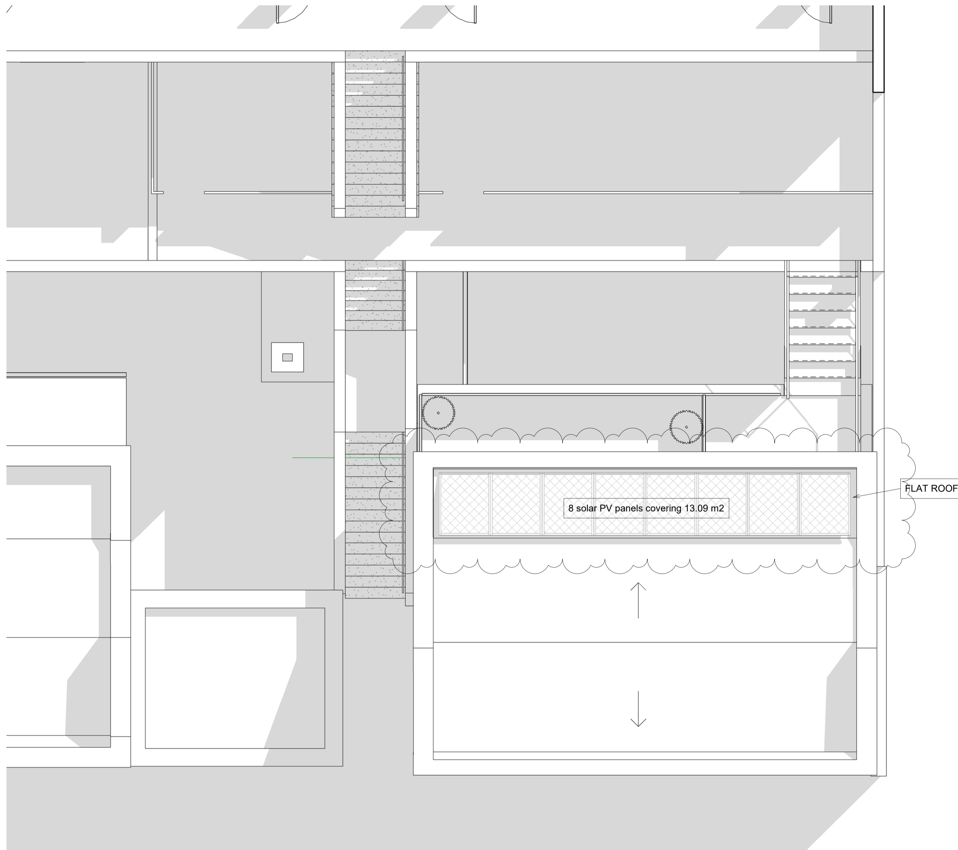
1 Proposed Roof level 1:50
