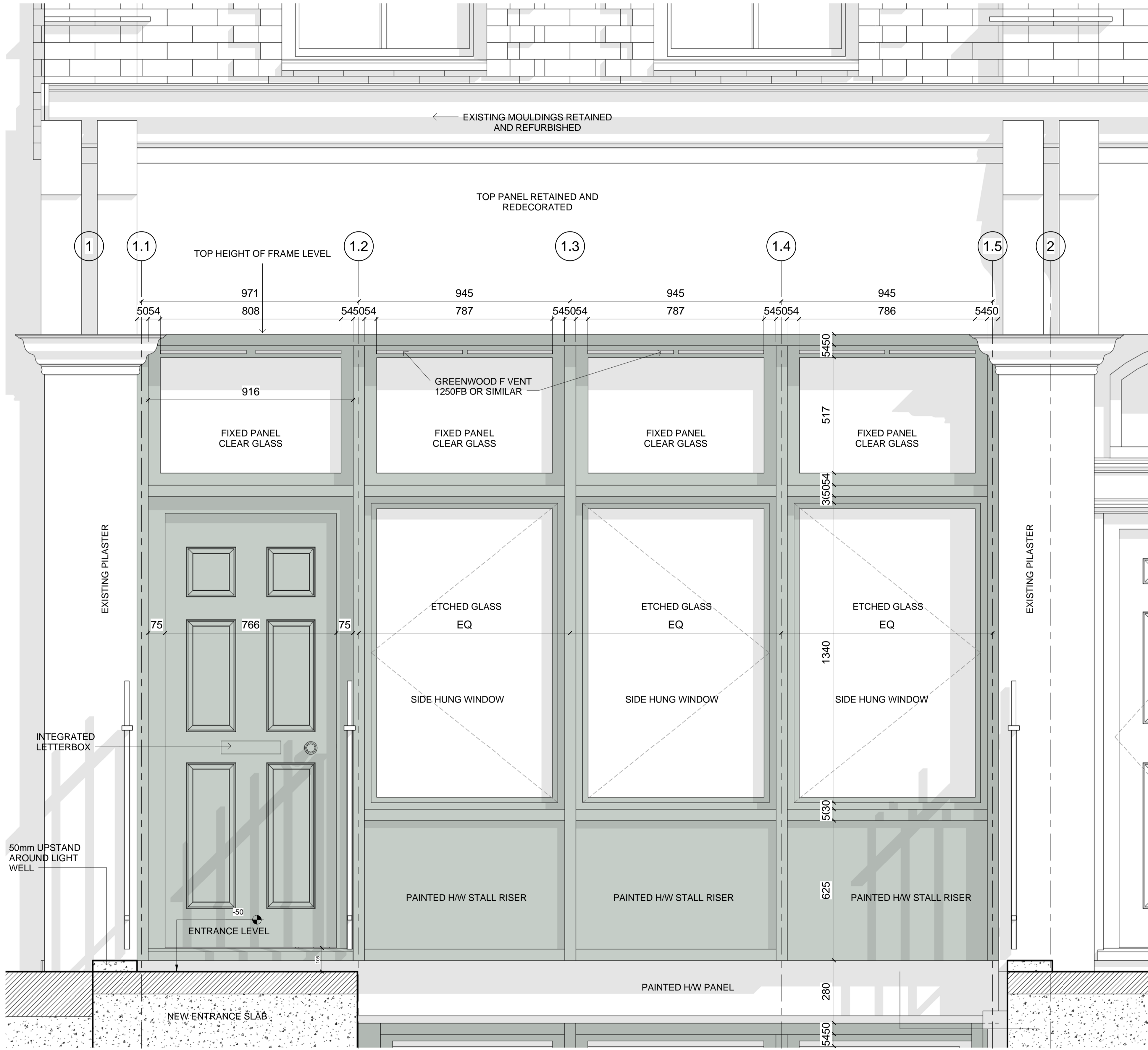
ELEVATION 1:10
