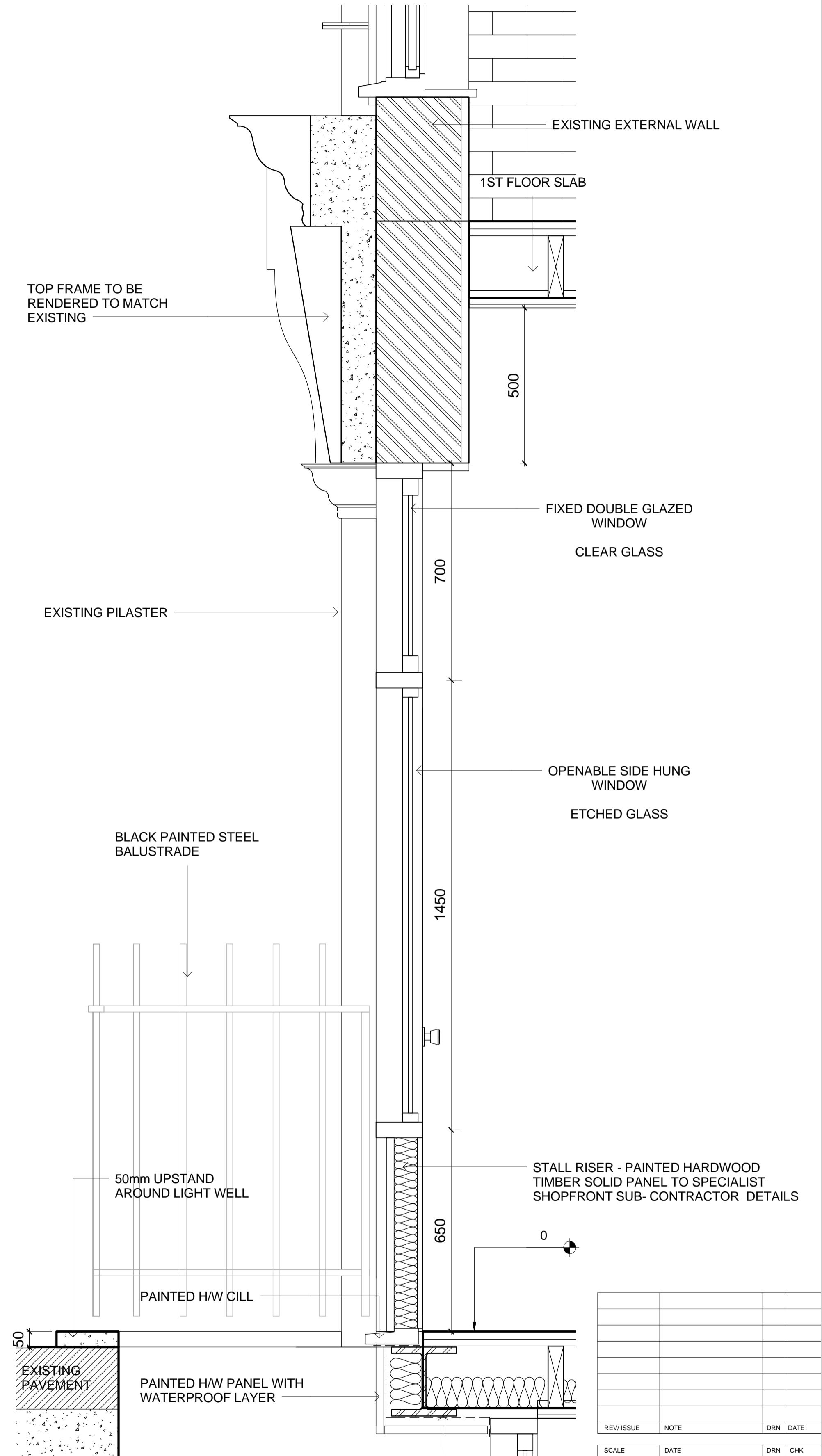
SECTION 1:10
