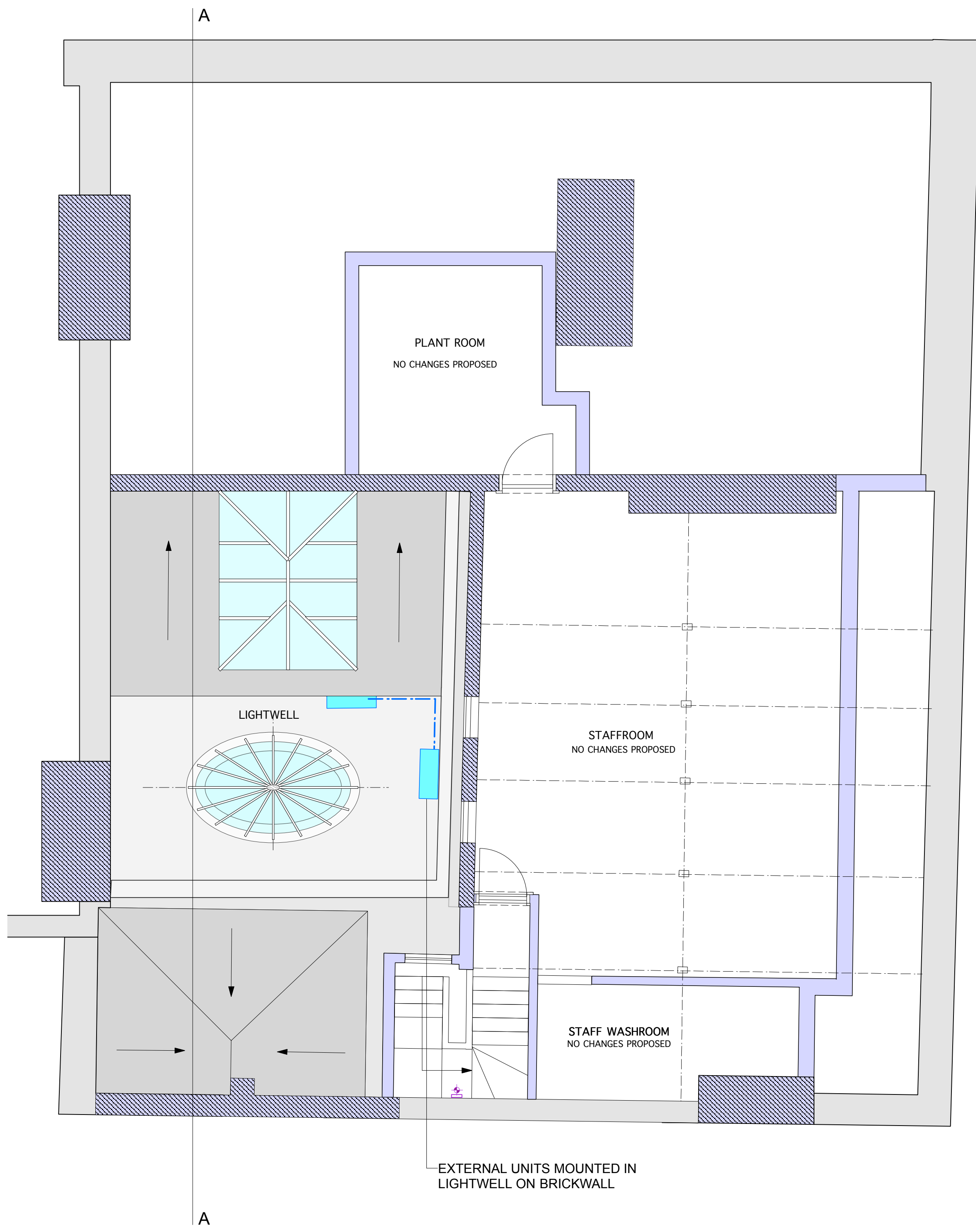
LOFT LAYOUT
