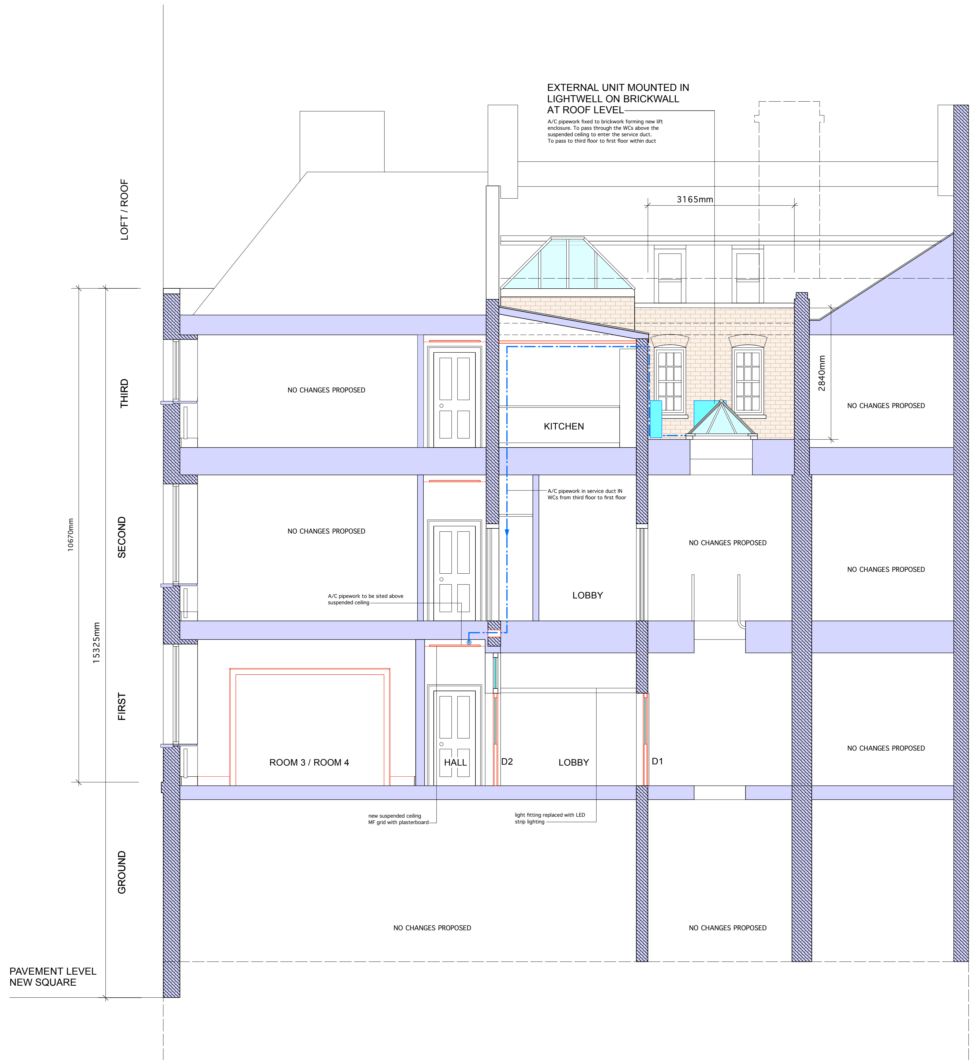
SECTION AA (DETAIL)
