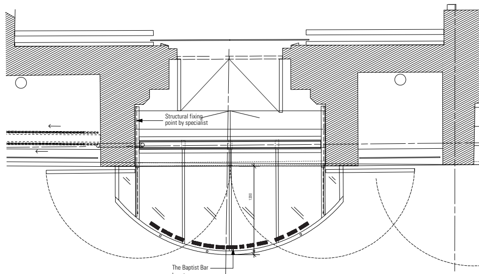
3 Plan View Ground Floor 1:25@A1, 1:50@A3
