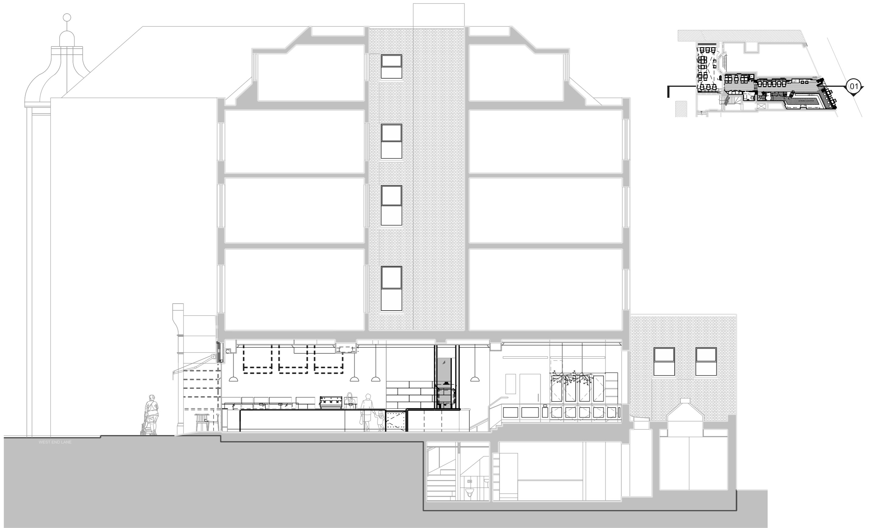
01 EXISTING SECTION BB 1:100
