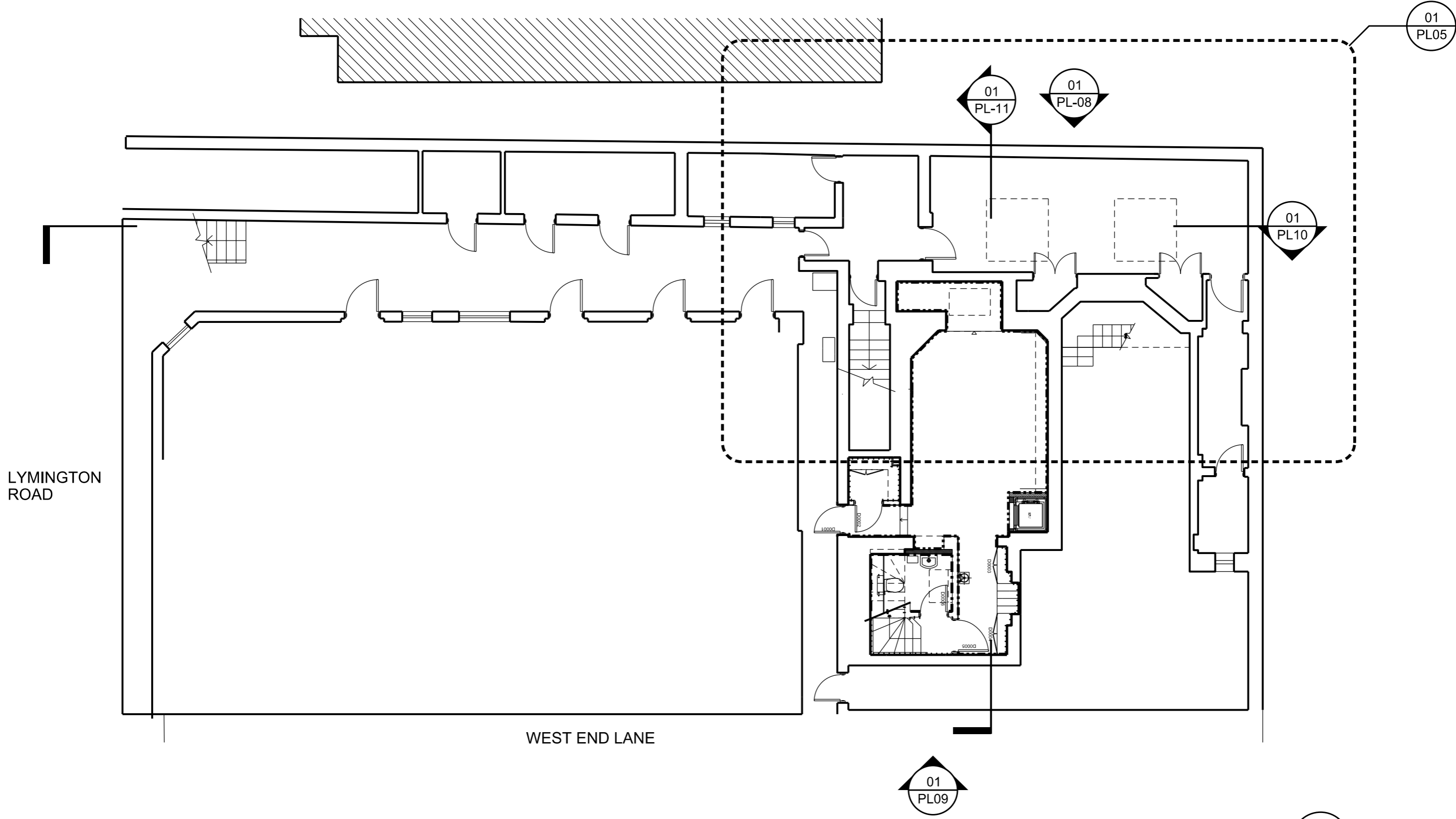
01 EXISTING LOWER GROUND FLOOR GA 1:100
