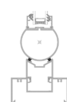
AFT Hinge Stile Detail
