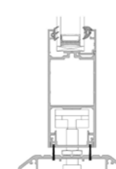
Threshold Detail
