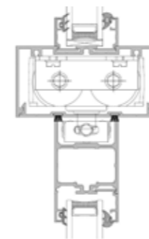
Transom Detail
