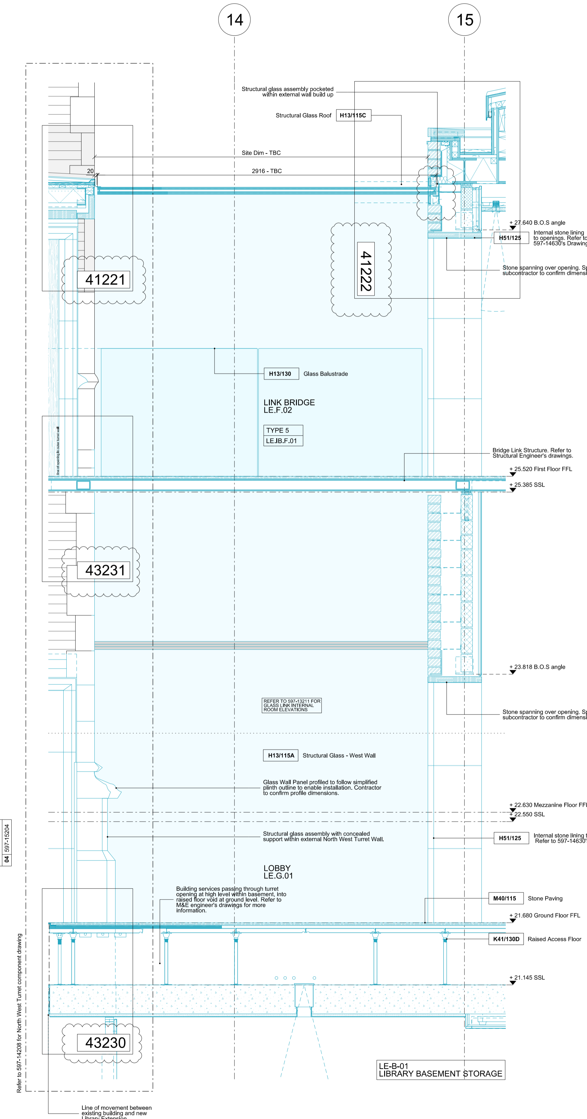
Glazed Link Cranked Section X-X 1:20 04 597-15204
