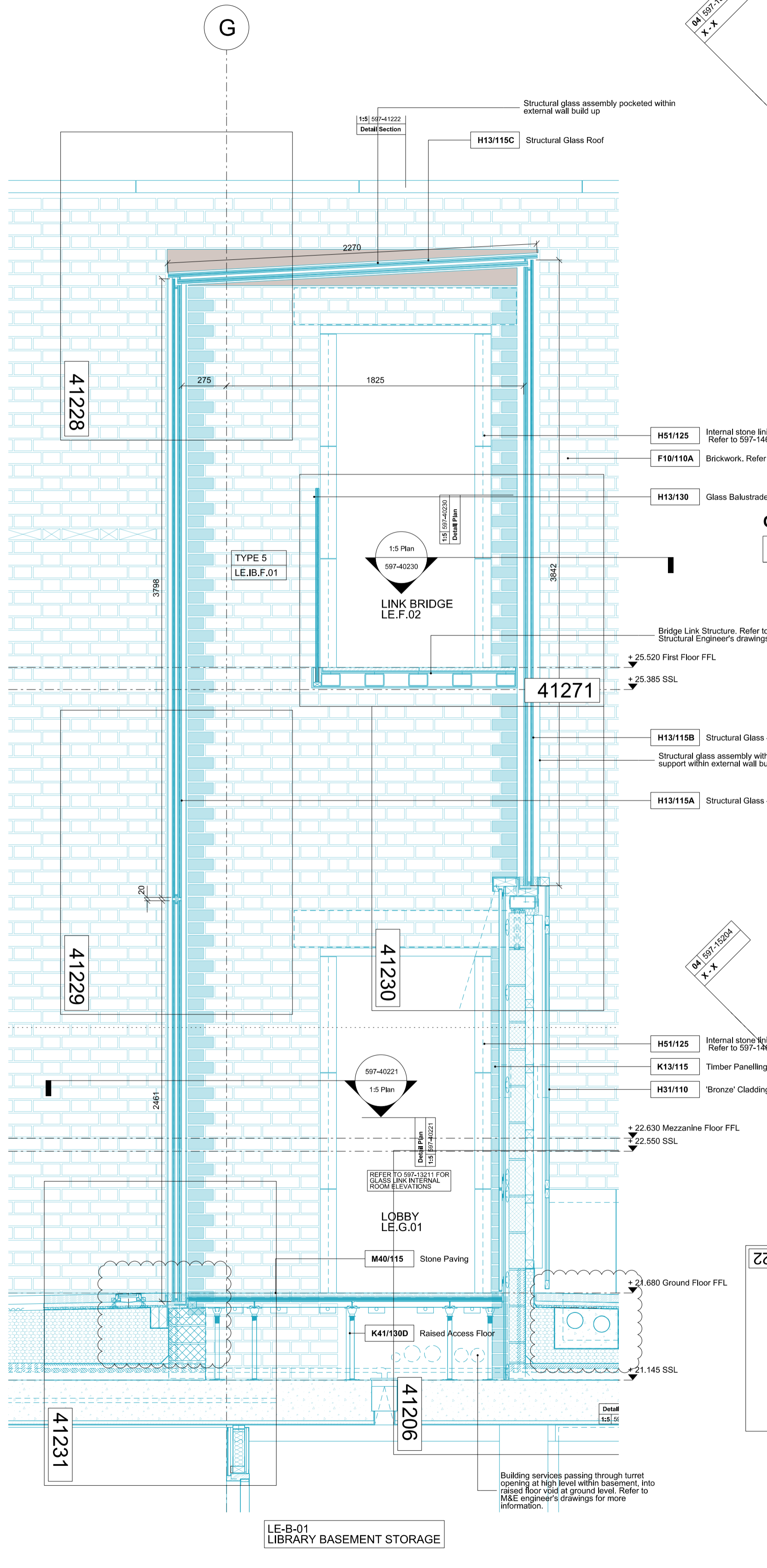
Glazed Link Section O-O' 1:20 01 597-15204
