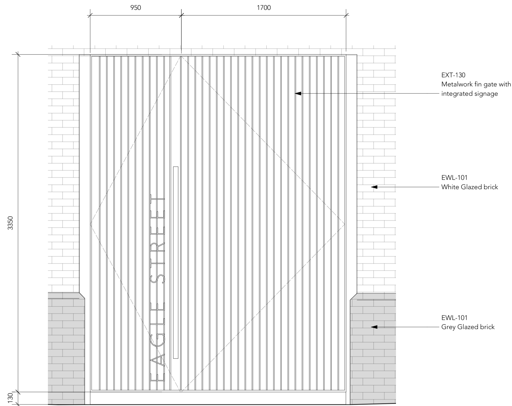
1 Gate Elevation 1:25
