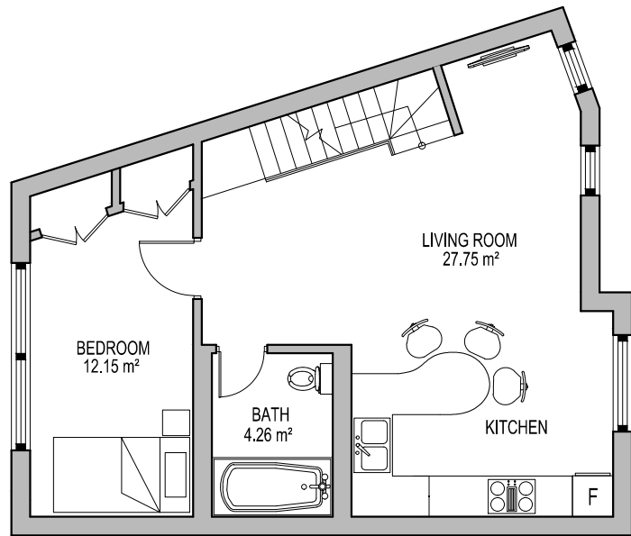
PROPOSED SECOND FLOOR 49.53 m²
