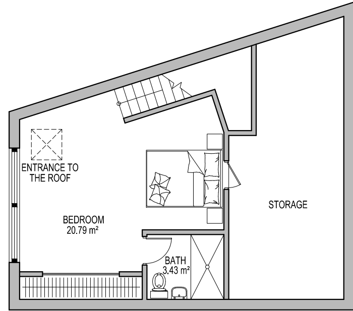
PROPOSED THIRD FLOOR 27.03 m²
