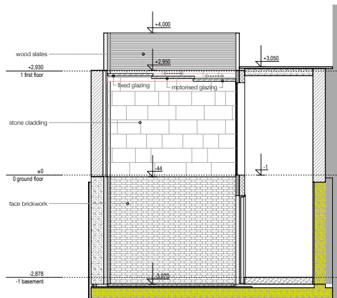
NORTH ELEVATION
