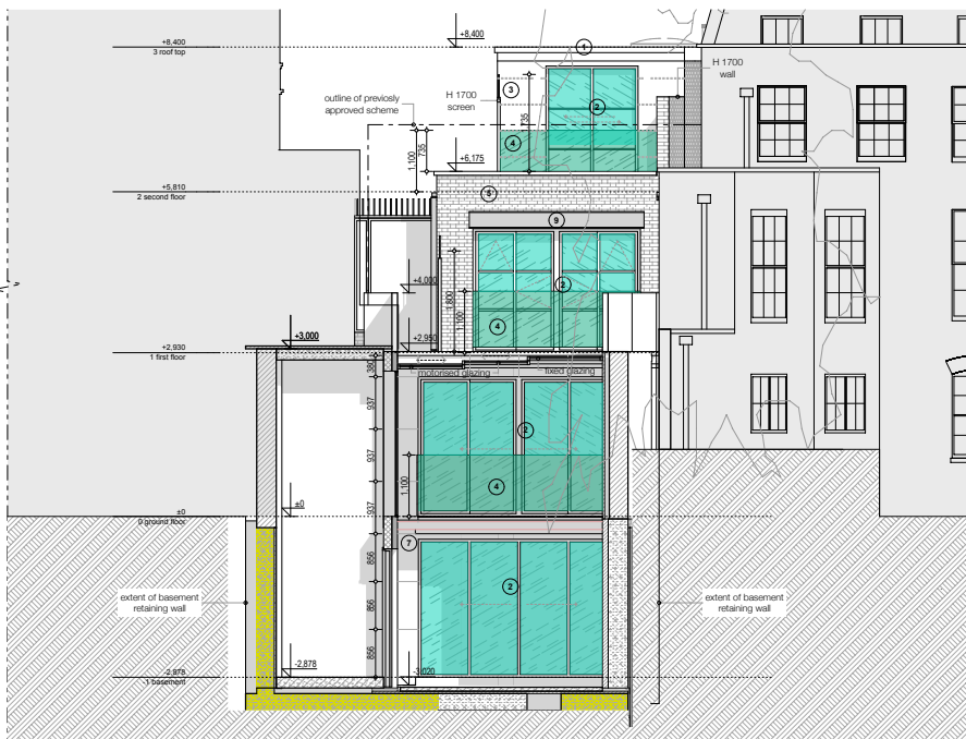
rear elevation as proposed NW 1:50
