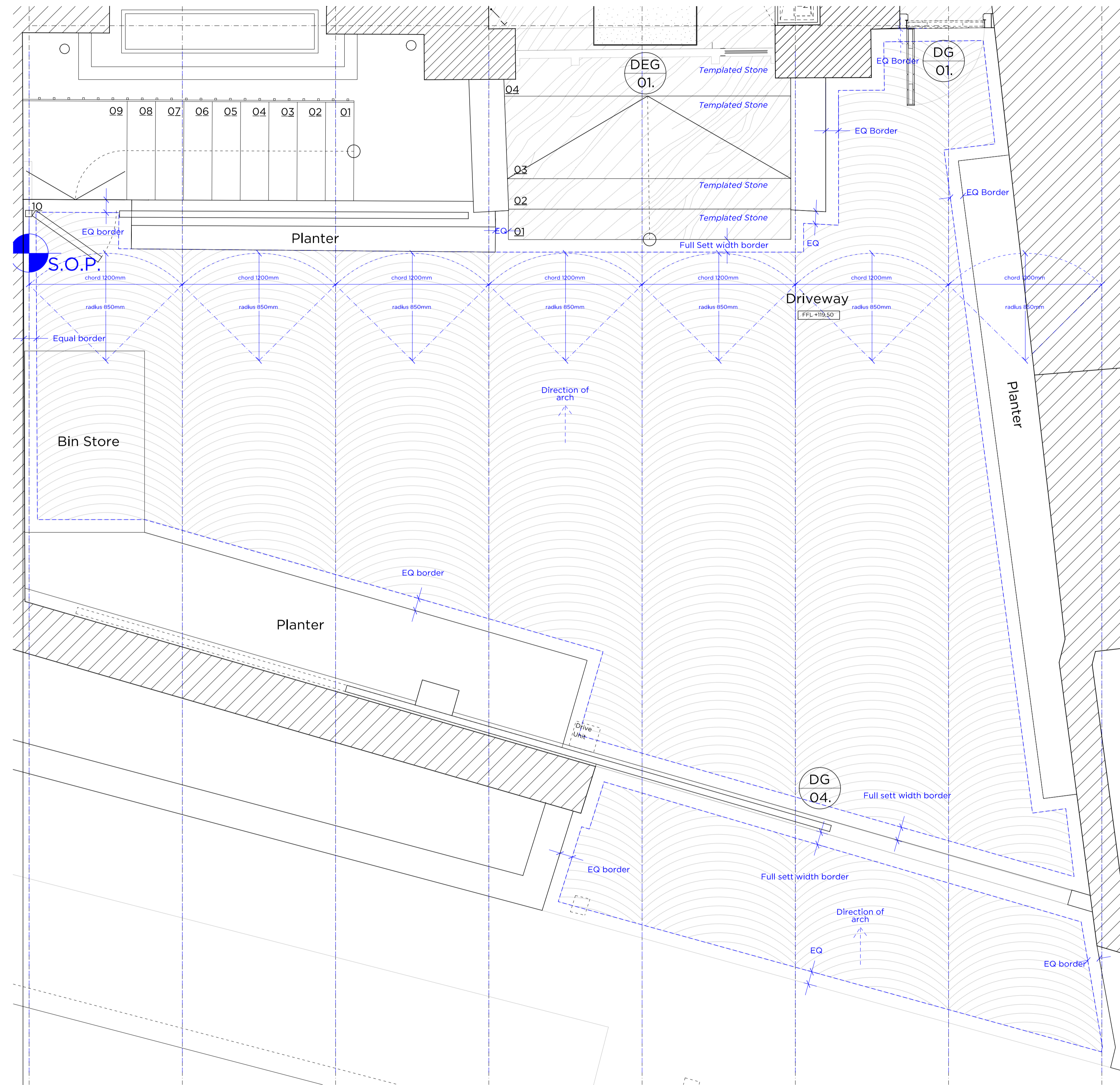
200_501 01 Front Garden_Stone Setting Out 1:20
