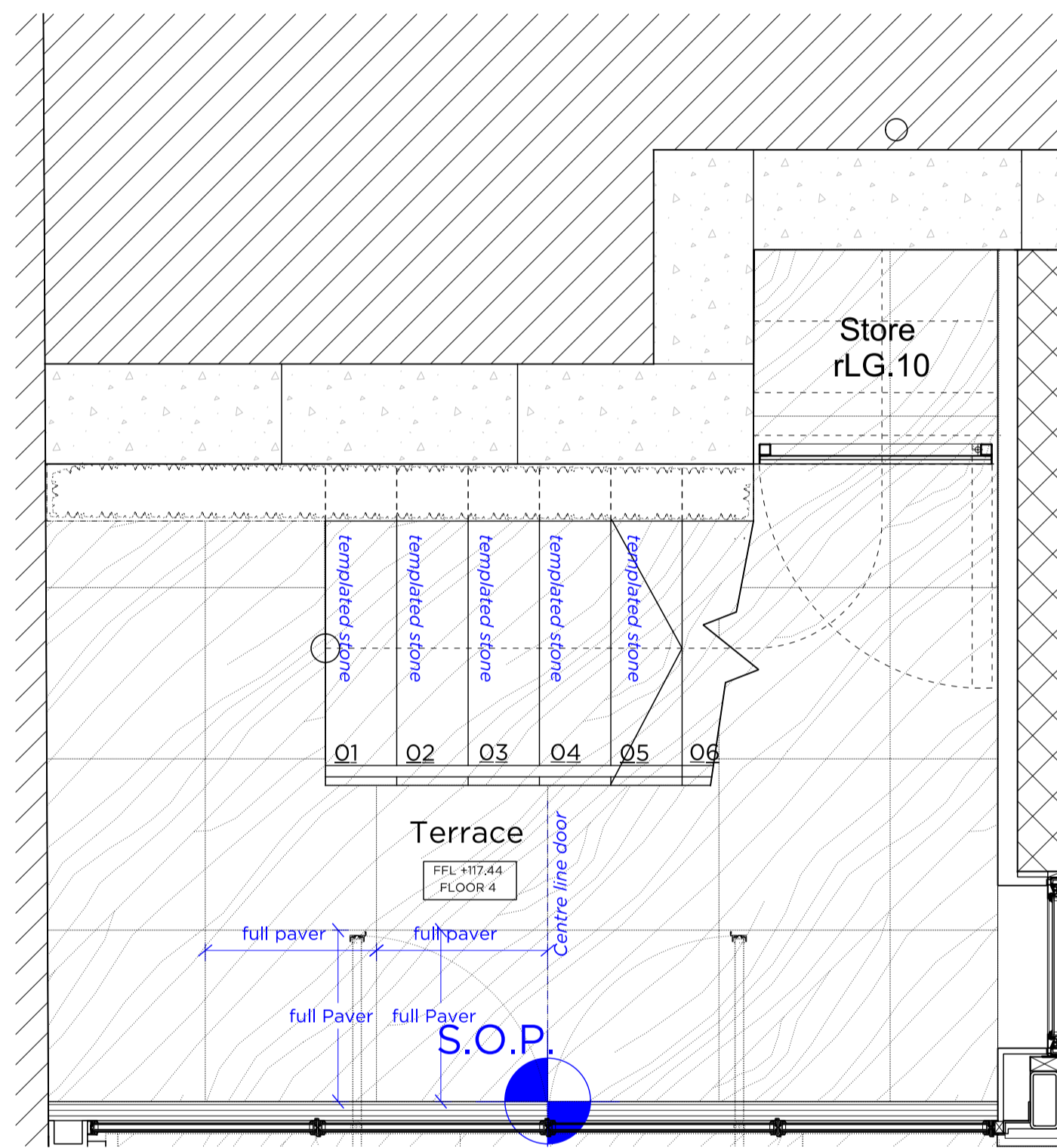
200_503 Rear Patio_Stone Setting Out 01 1:20
