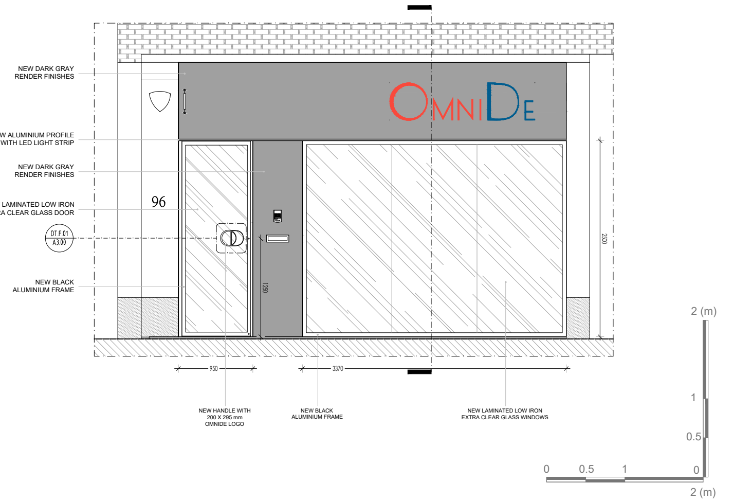
2 PROPOSED ELEVATION, scale 1:50@A3
