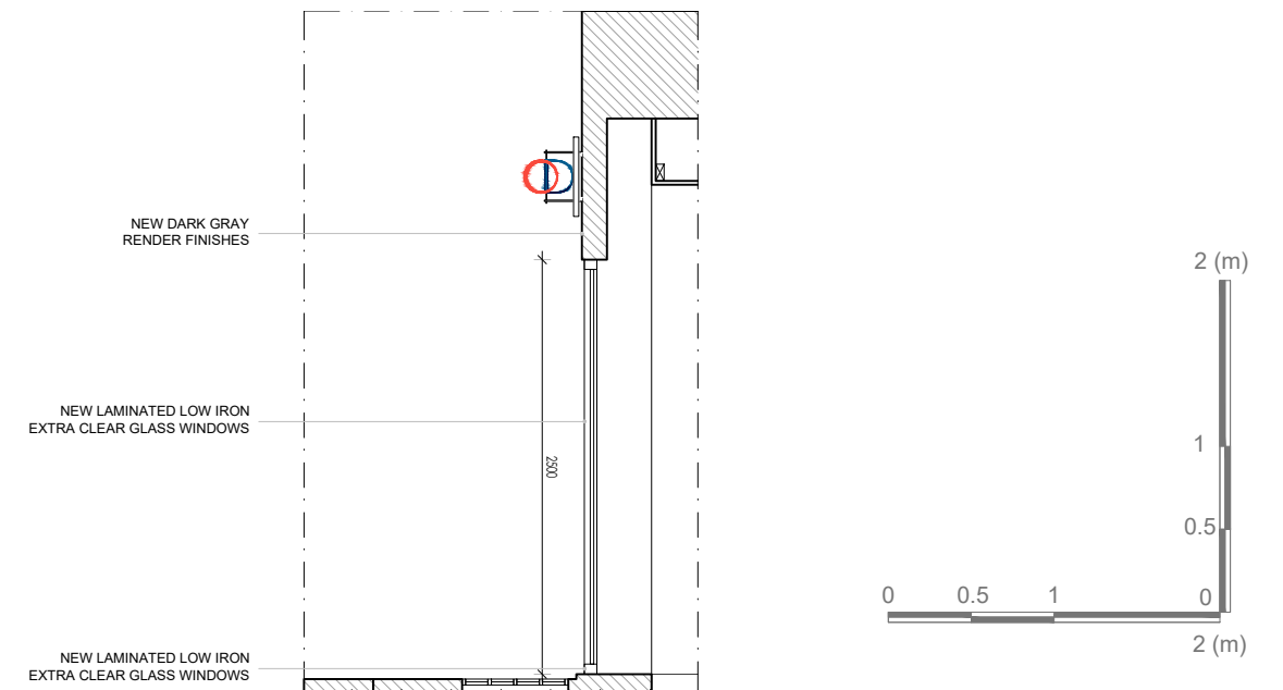
4 PROPOSED SECTION, scale 1:50@A3
