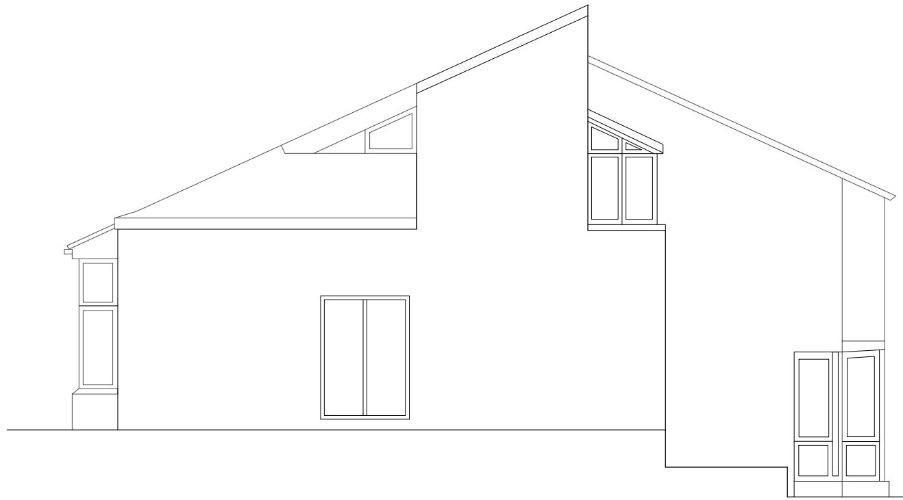
RIGHT SIDE / EAST ELEVATION
