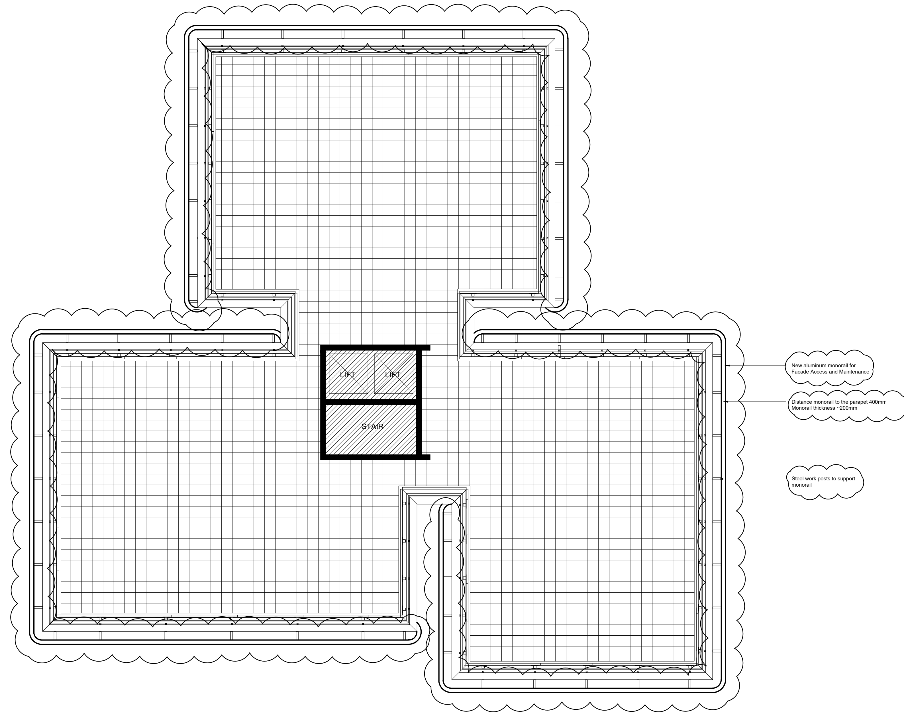
1- Plan - Existing Roof Plan Scale 1 : 100
