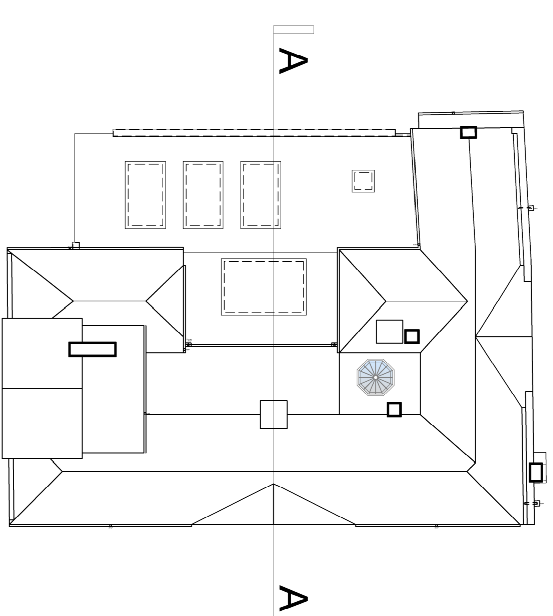
Existing key roof plan nts
