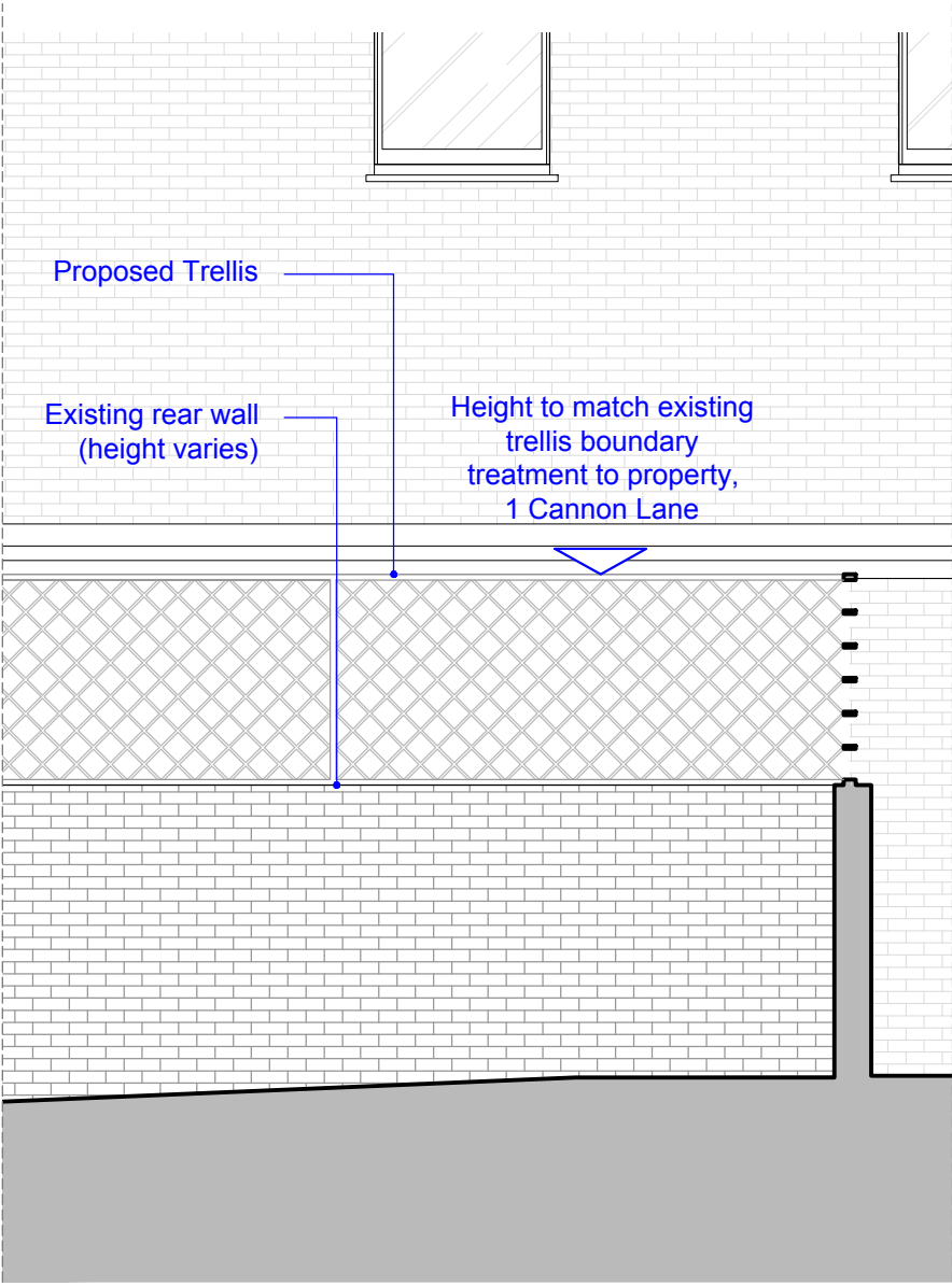
02 TRELLIS SECTION SCALE 1:50
