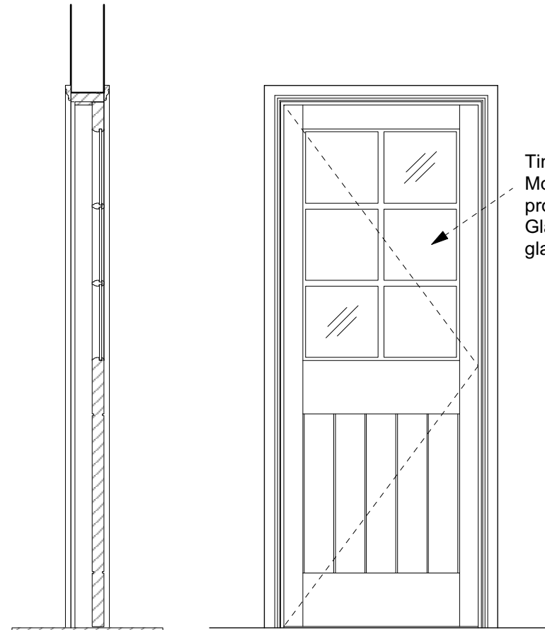
Section 1:20
