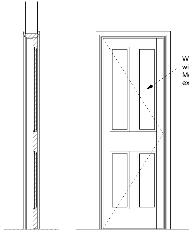
Section 1:20
