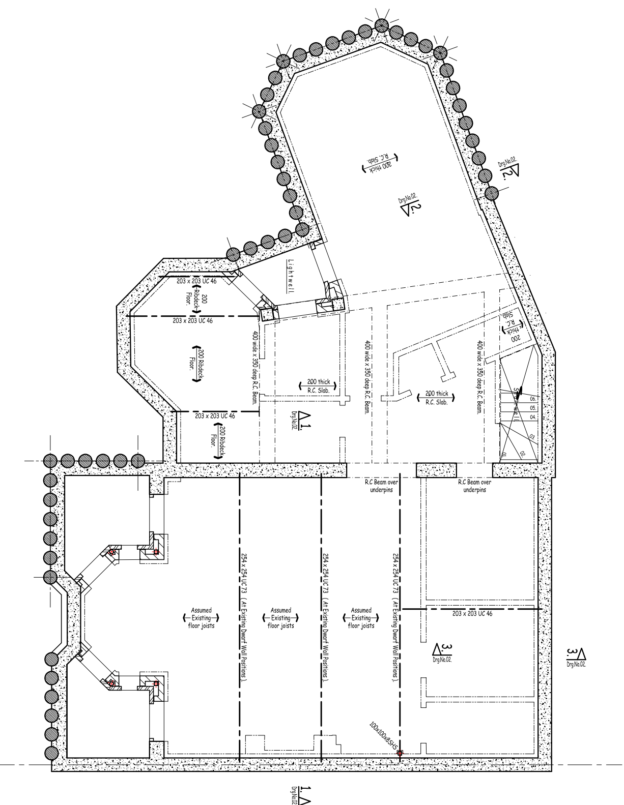
Proposed Basement Plan Showing Ground Floor Structure.
