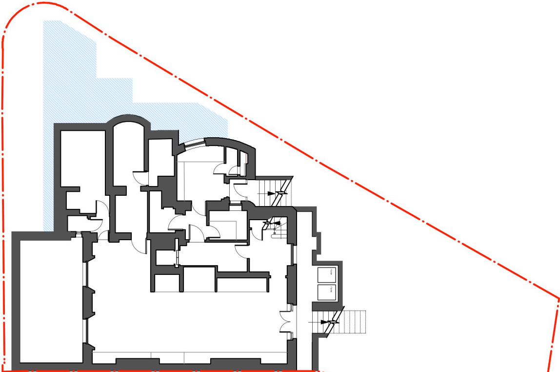
PROPOSED EXTENSION TO LOWER GROUND FLOOR - 33 SQM
