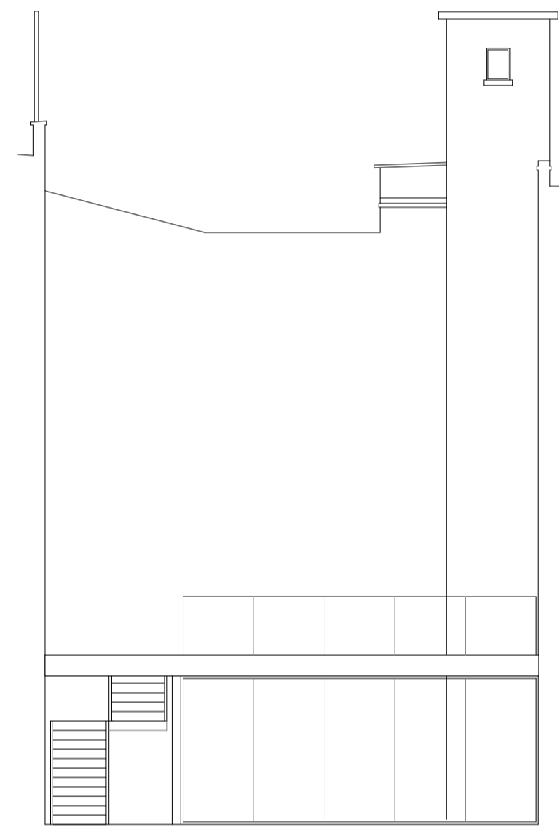
LIGHT WELL ELEVATION _ 1
