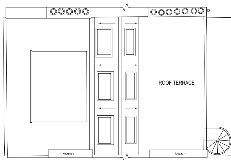
ROOF PLAN FLAT 2
