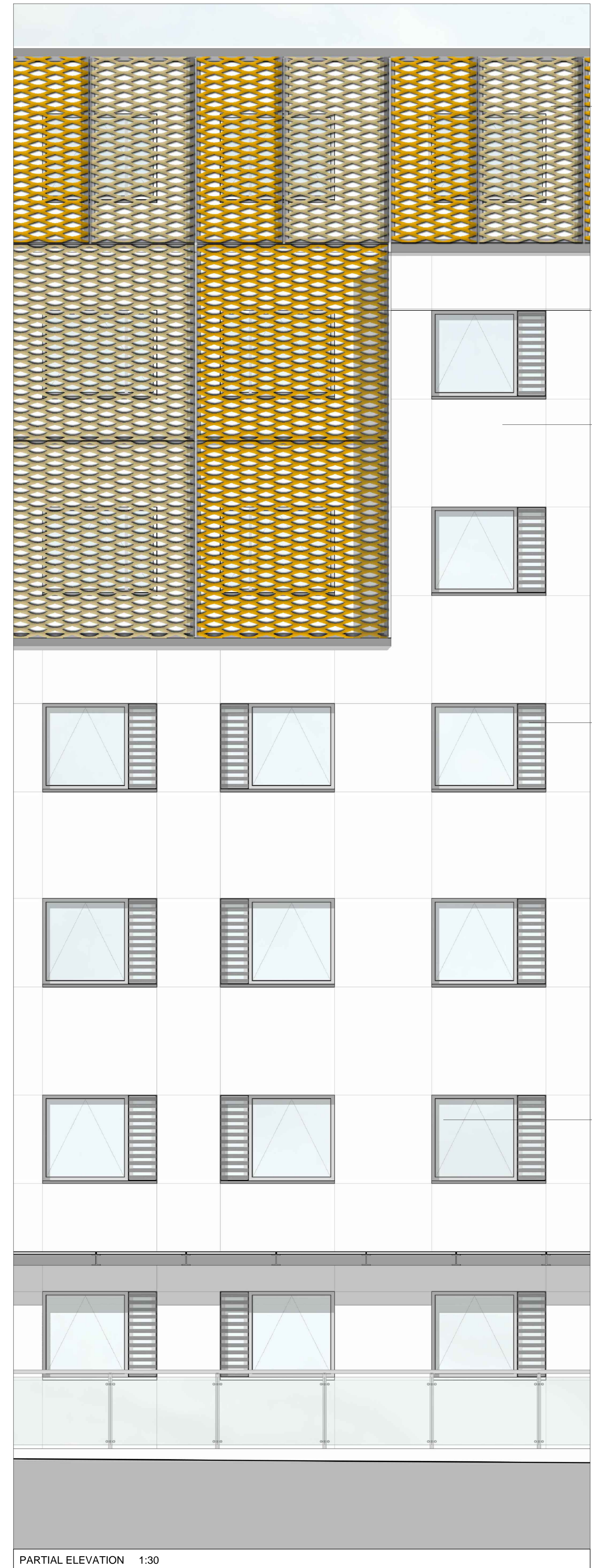
PARTIAL ELEVATION 1:30
