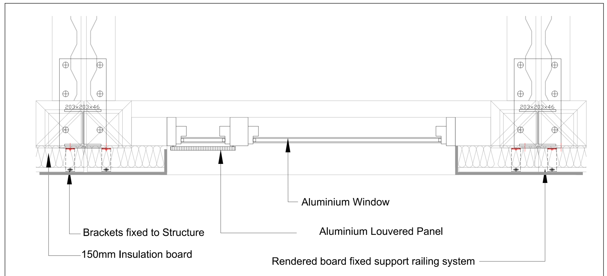
WINDOW PLAN DETAIL S. 1:10
