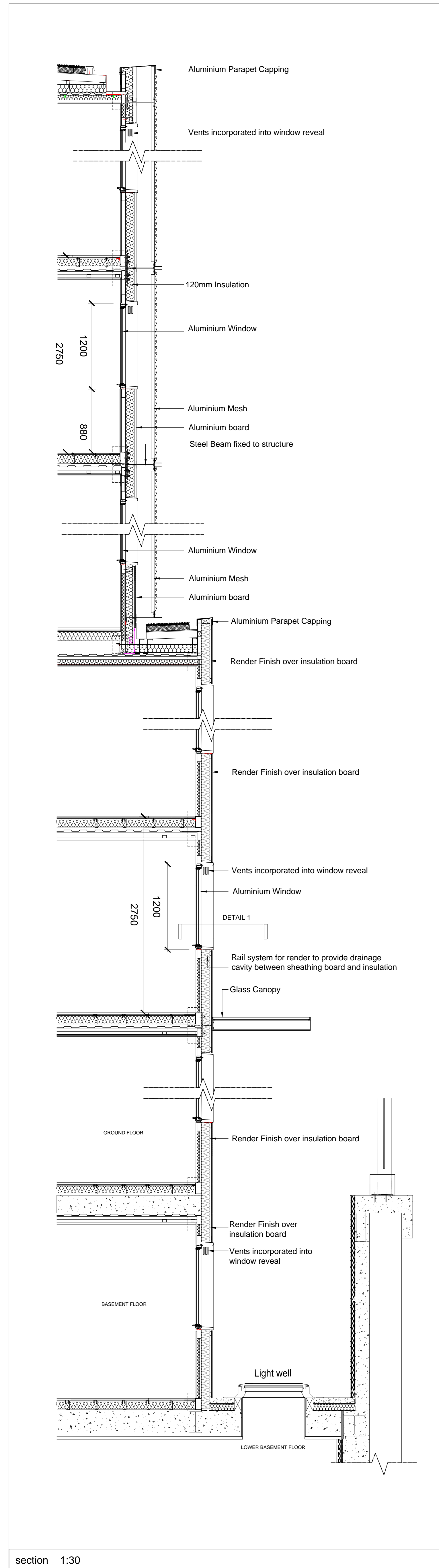
section 1:30
