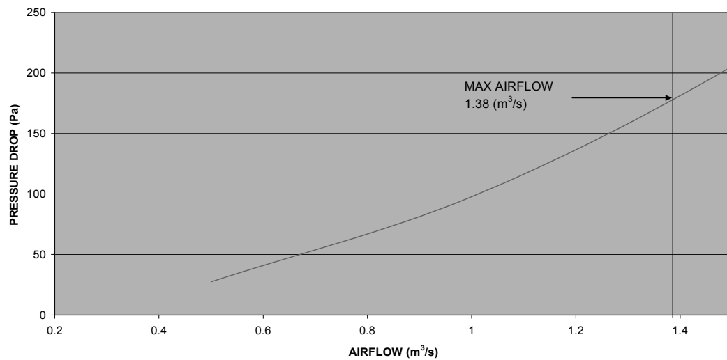
RESISTANCE AGAINST AIRFLOW ESP3000E
