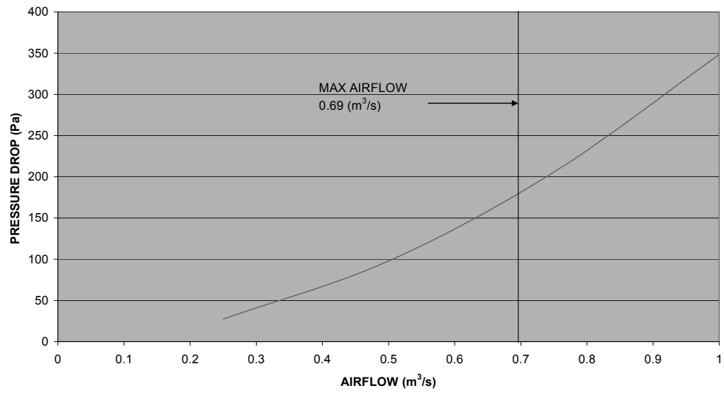
RESISTANCE AGAINST AIRFLOW ESP1500E
