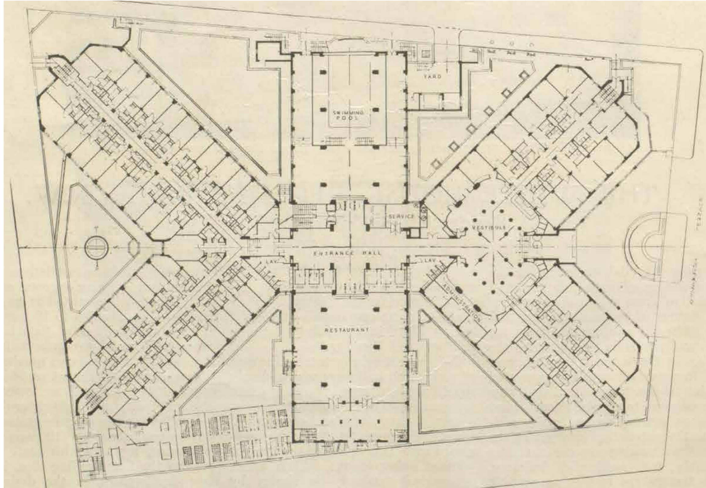
Original Ground Floor Plan
