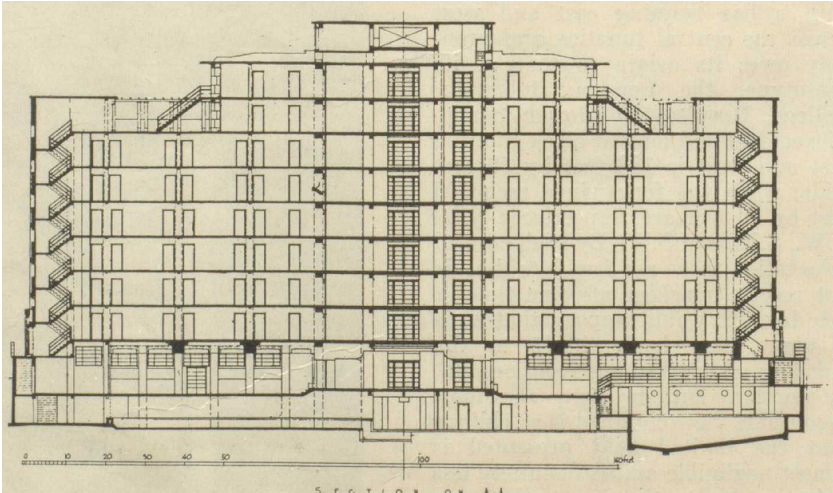
Cross Section West-east wings
