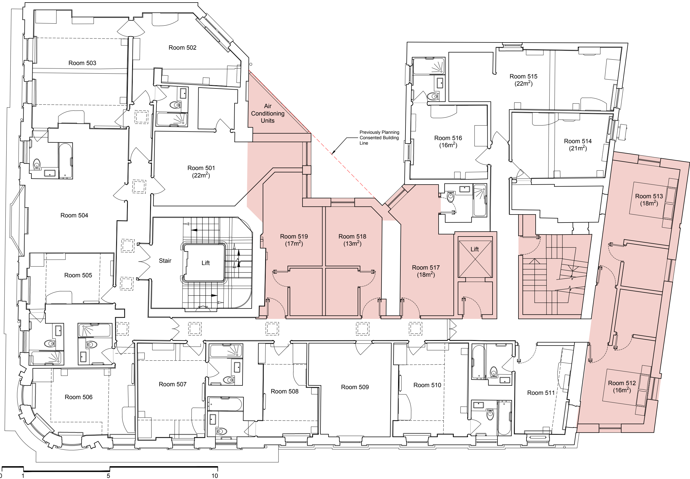
■ Proposal Proposed Fifth Floor Scale 1:100
