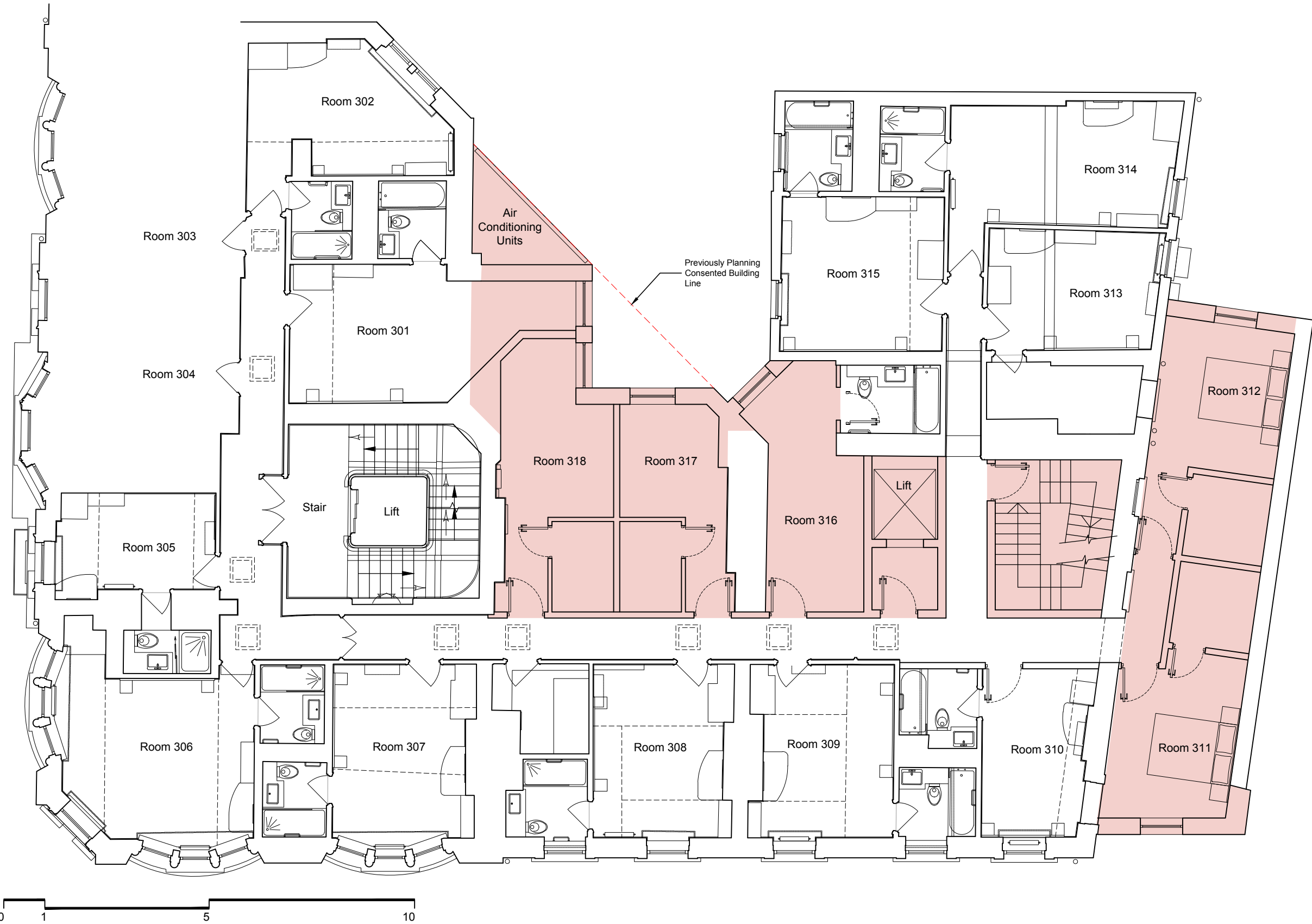
Proposed Third Floor Scale 1:100
