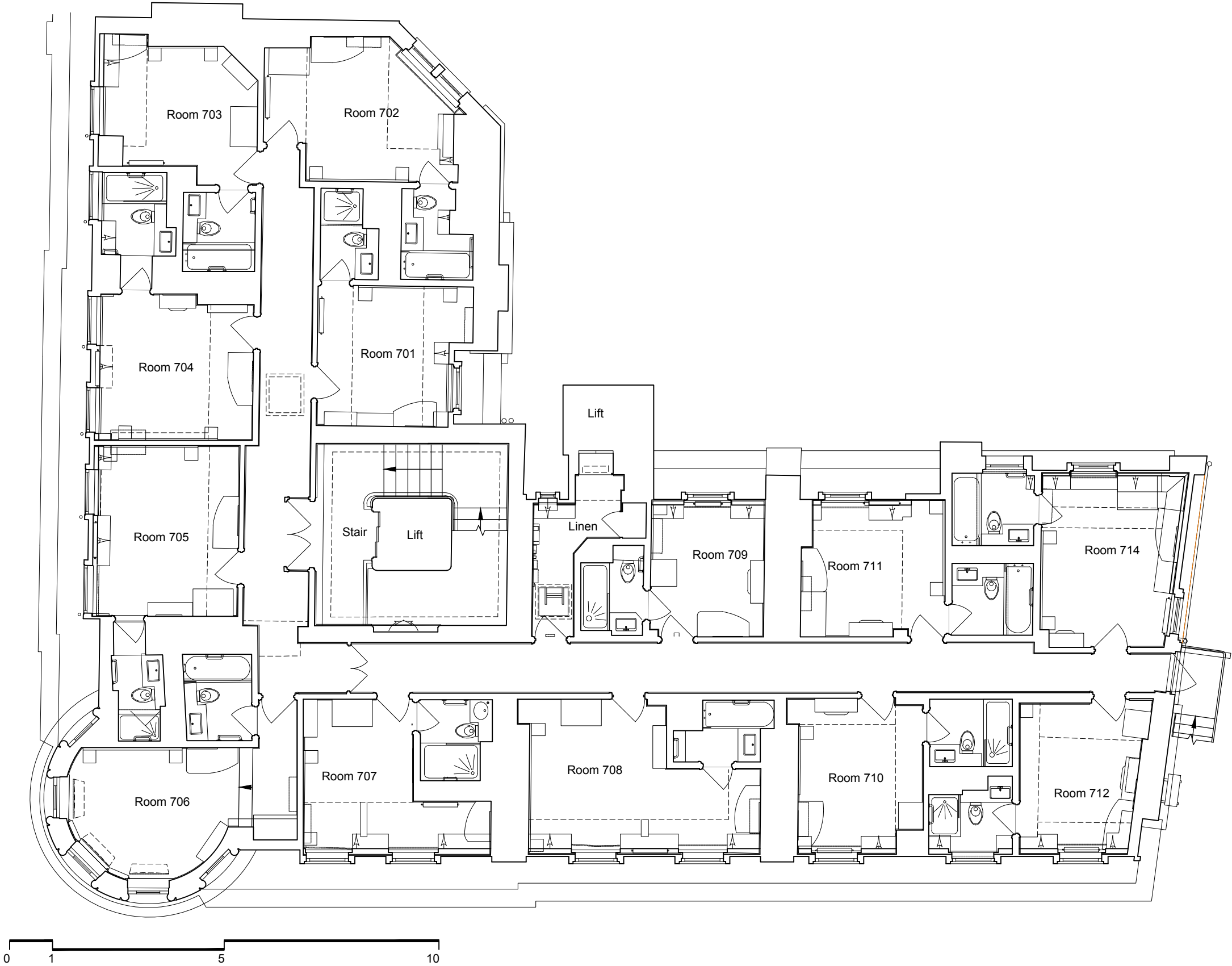
Existing Seventh Floor Scale 1:100
