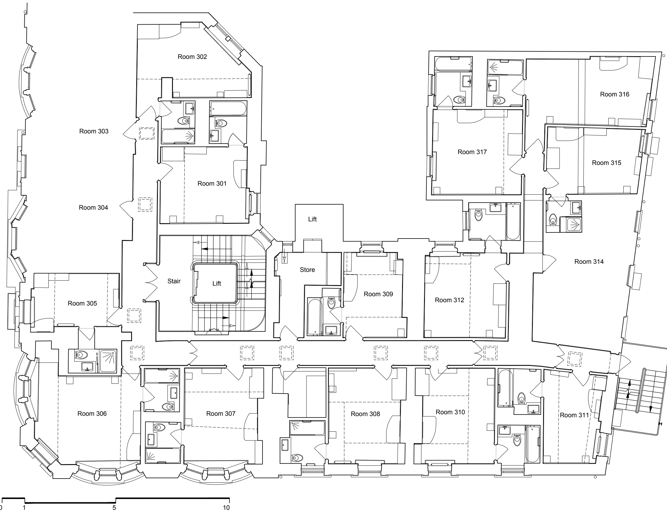
Existing Third Floor Scale 1:100
