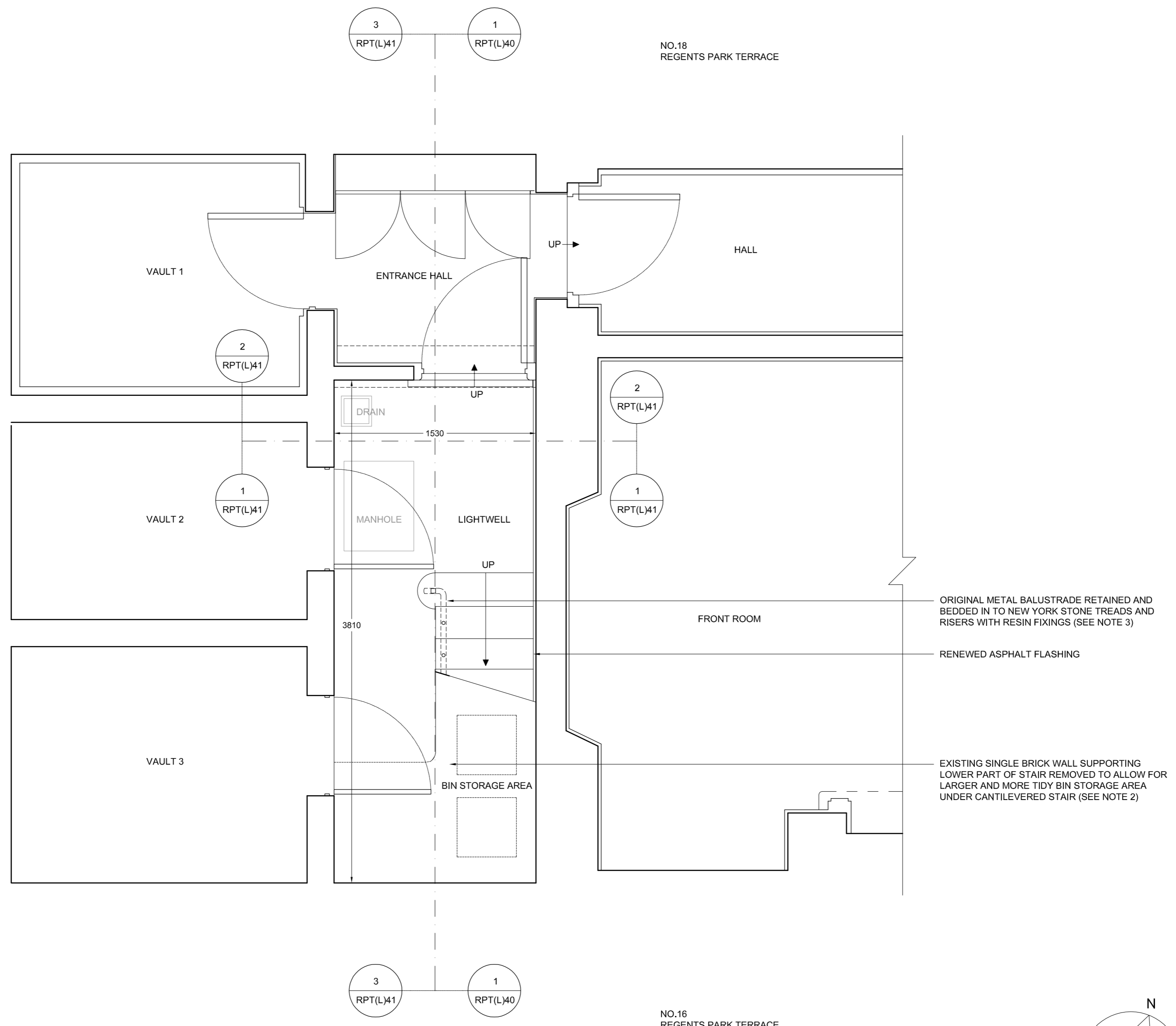
LOWER GROUND FLOOR LEVEL PLAN OF LIGHTWELL AND VAULT AREA - AS PROPOSED
