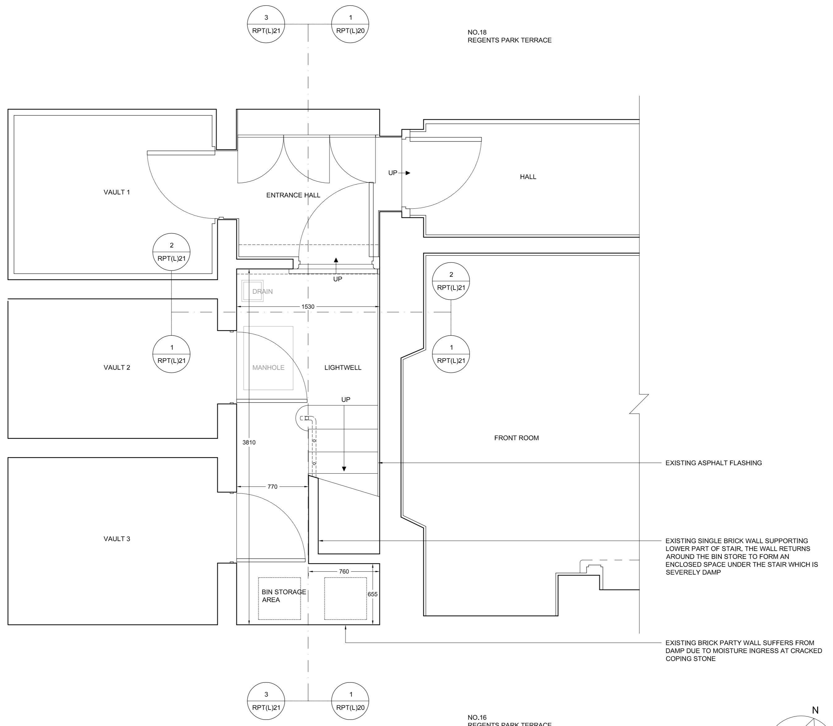
1 RPT(L)10 LOWER GROUND FLOOR LEVEL PLAN OF LIGHTWELL AND VAULT AREA - AS EXISTING
